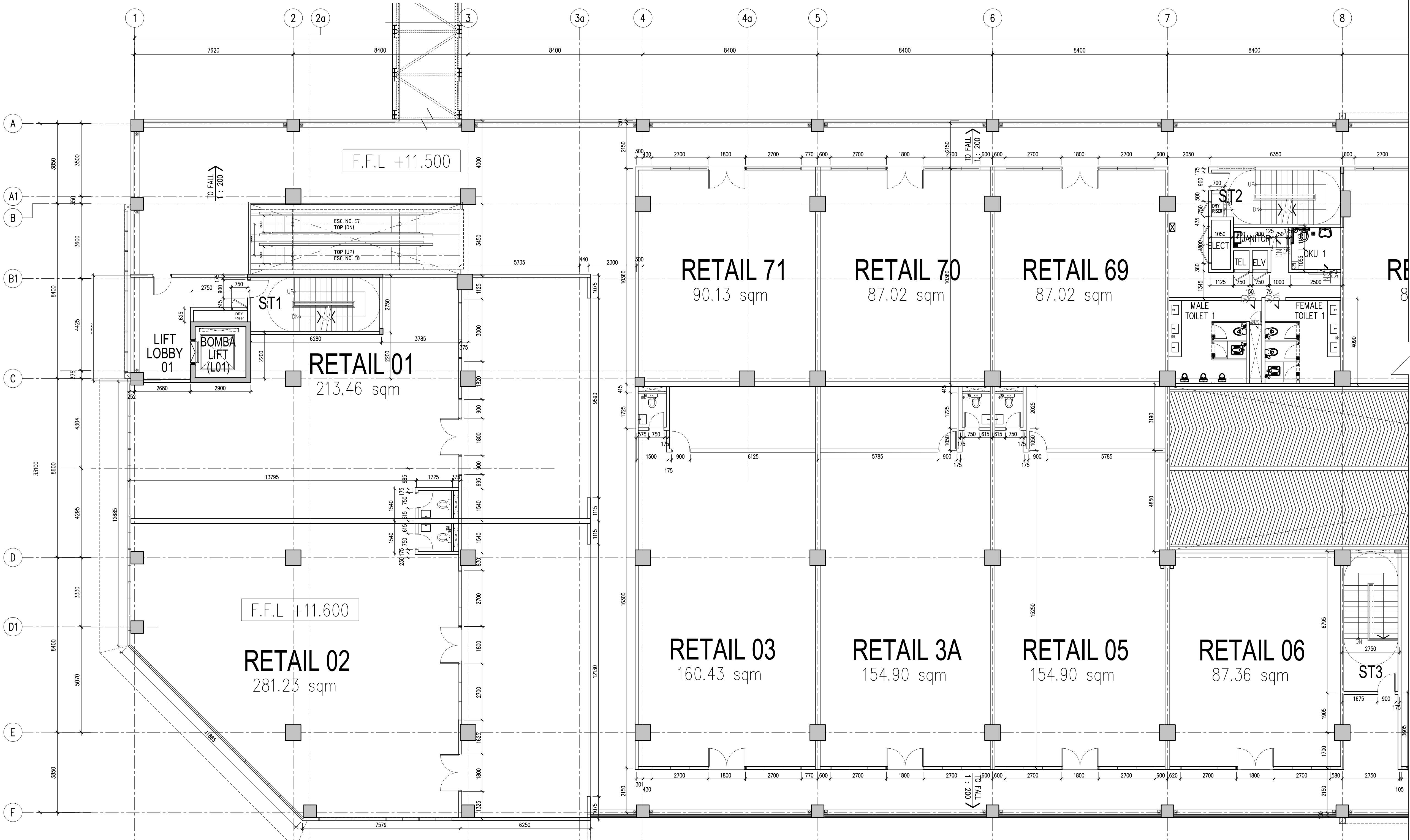
01 WALL SETTING OUT-LEVEL 3 PART 1 871-15 SCALE = 1 : 100
