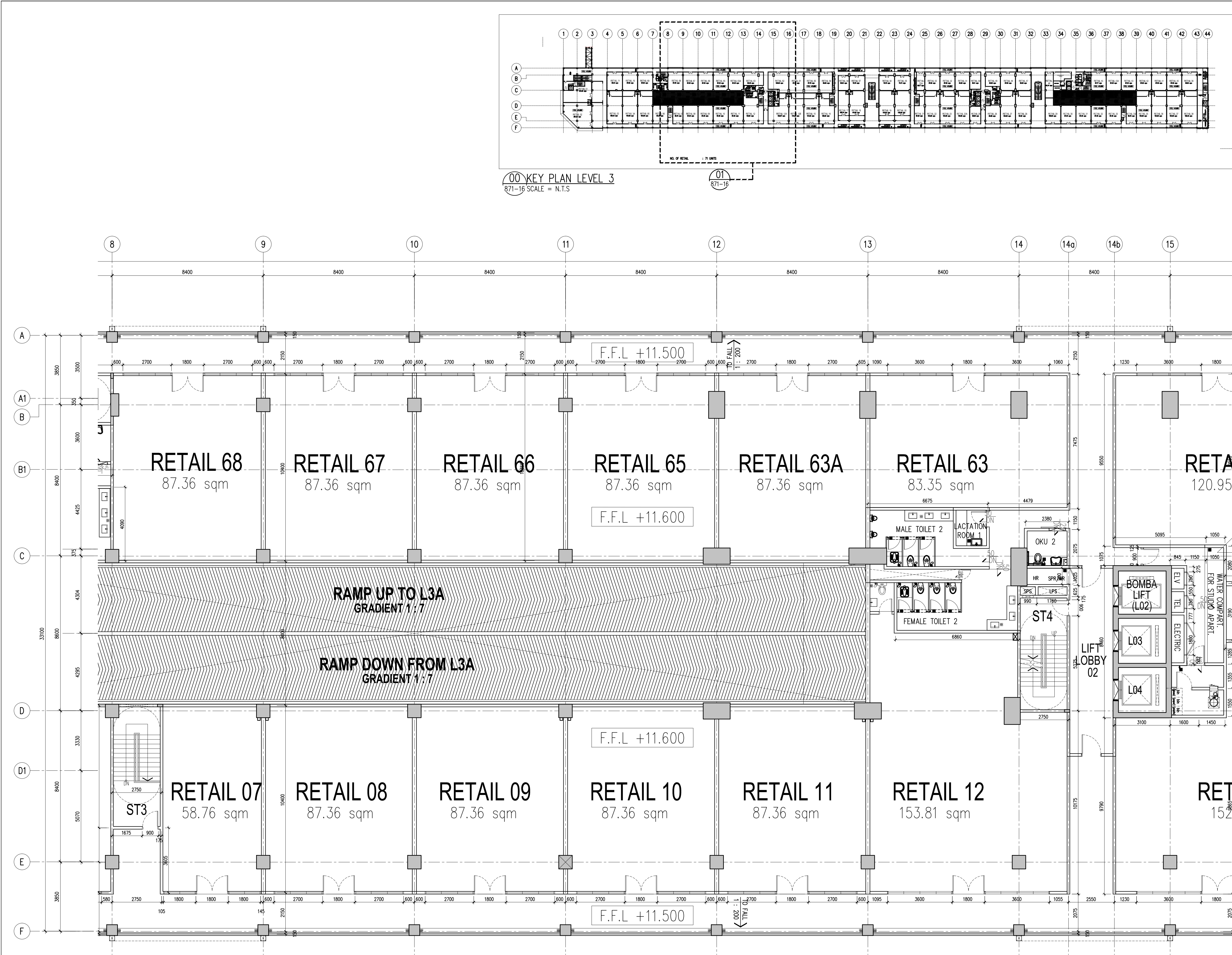
01 WALL SETTING OUT-LEVEL 3 PART 1 871-16 SCALE = 1 : 100
