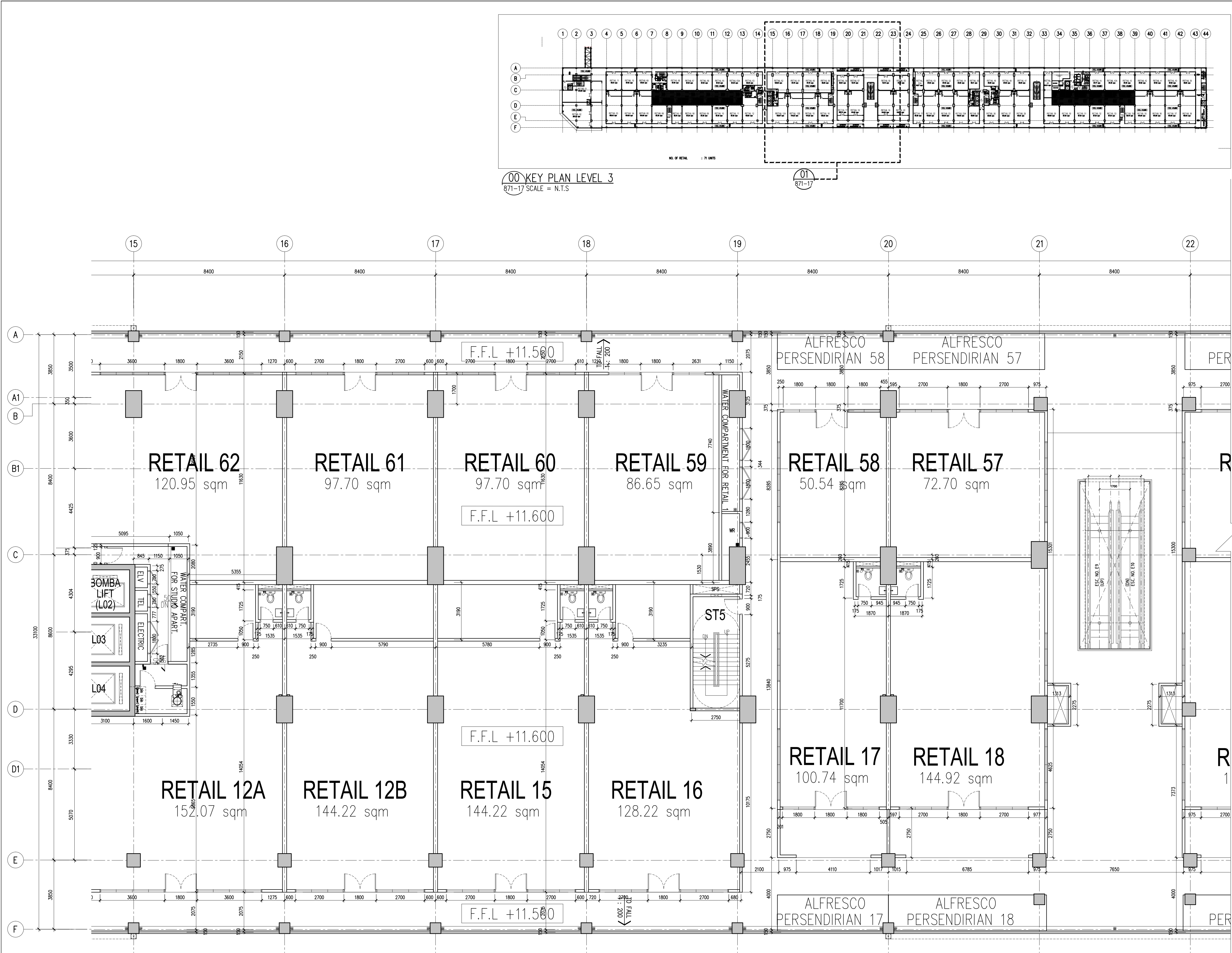
01 WALL SETTING OUT-LEVEL 3 PART 3 871-17 SCALE = 1 : 100 J:\project\555714_Batu Kawan Mixed development\LOT 11\557_07-FTP\FTP - OUT\2018_12_DEC_LATEST CONSTRUCTION AMENDMENT\557_CA-872-Wall Setting Out\acad(binded)\557_CA-871_15-21.dwg 06 Dec. 2018 - 4:37pm Shamsury
