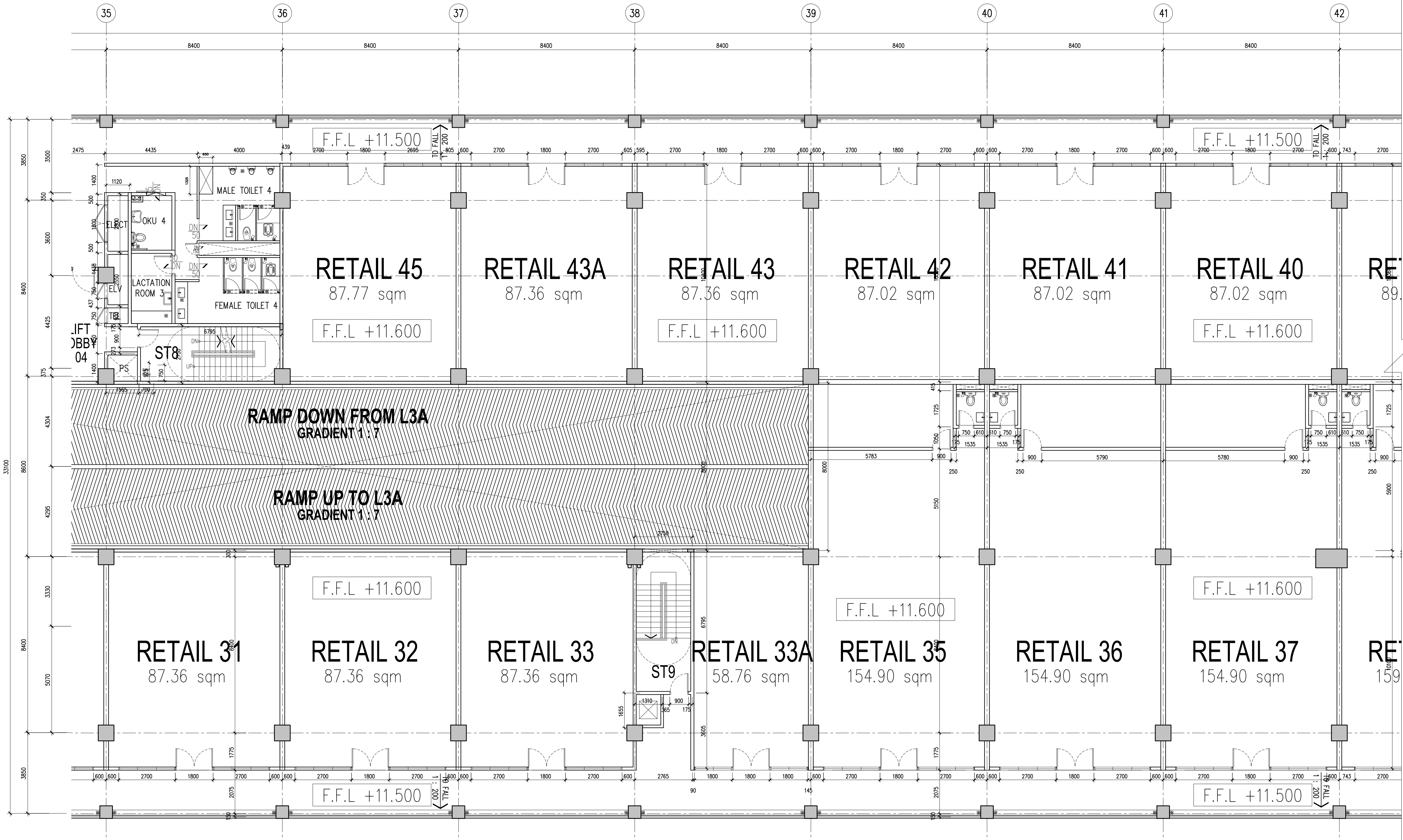
01 WALL SETTING OUT-LEVEL 3 PART 6 871-20 SCALE = 1 : 100
