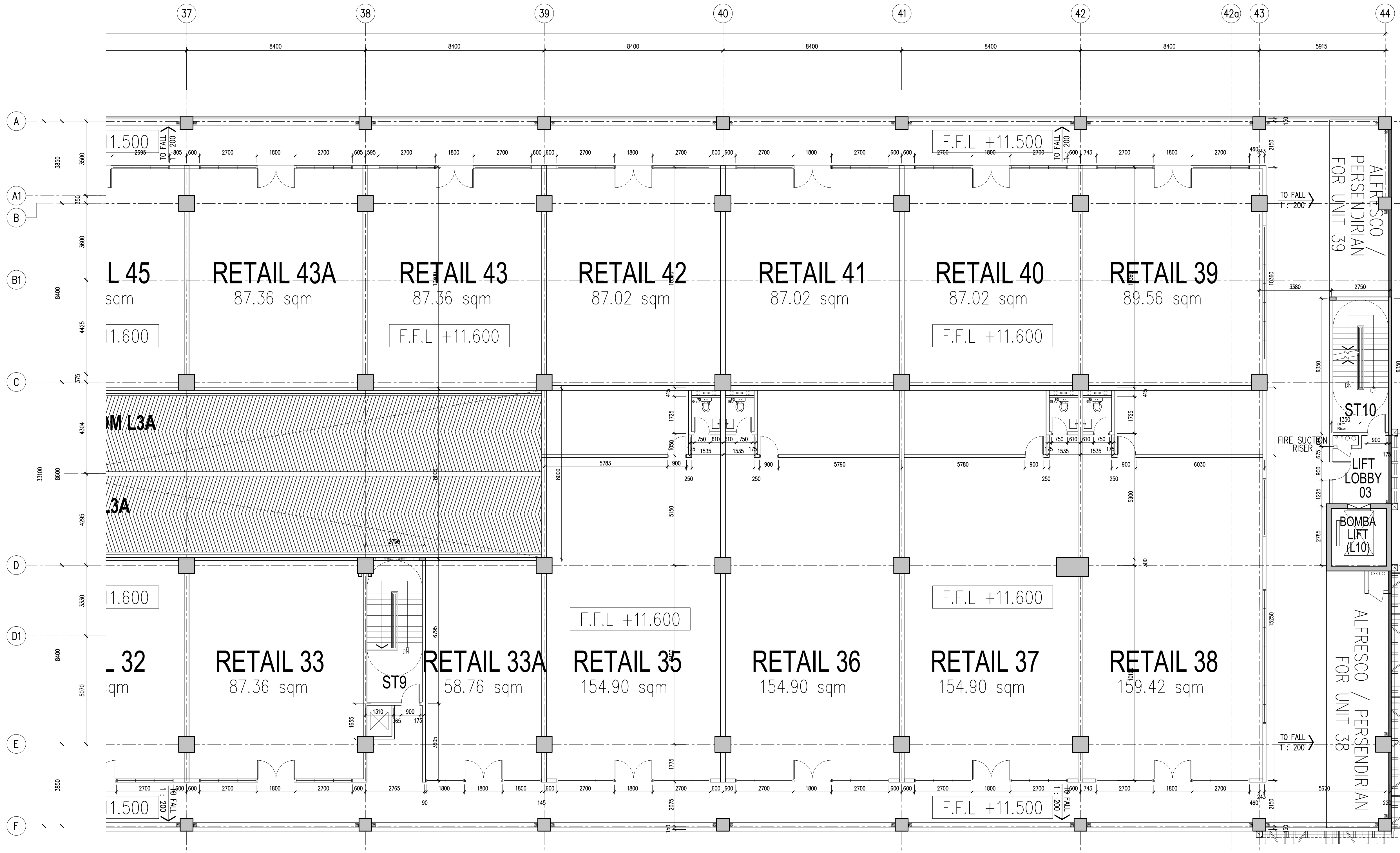
01 WALL SETTING OUT-LEVEL 3 PART 7 871-21 SCALE = 1 : 100
