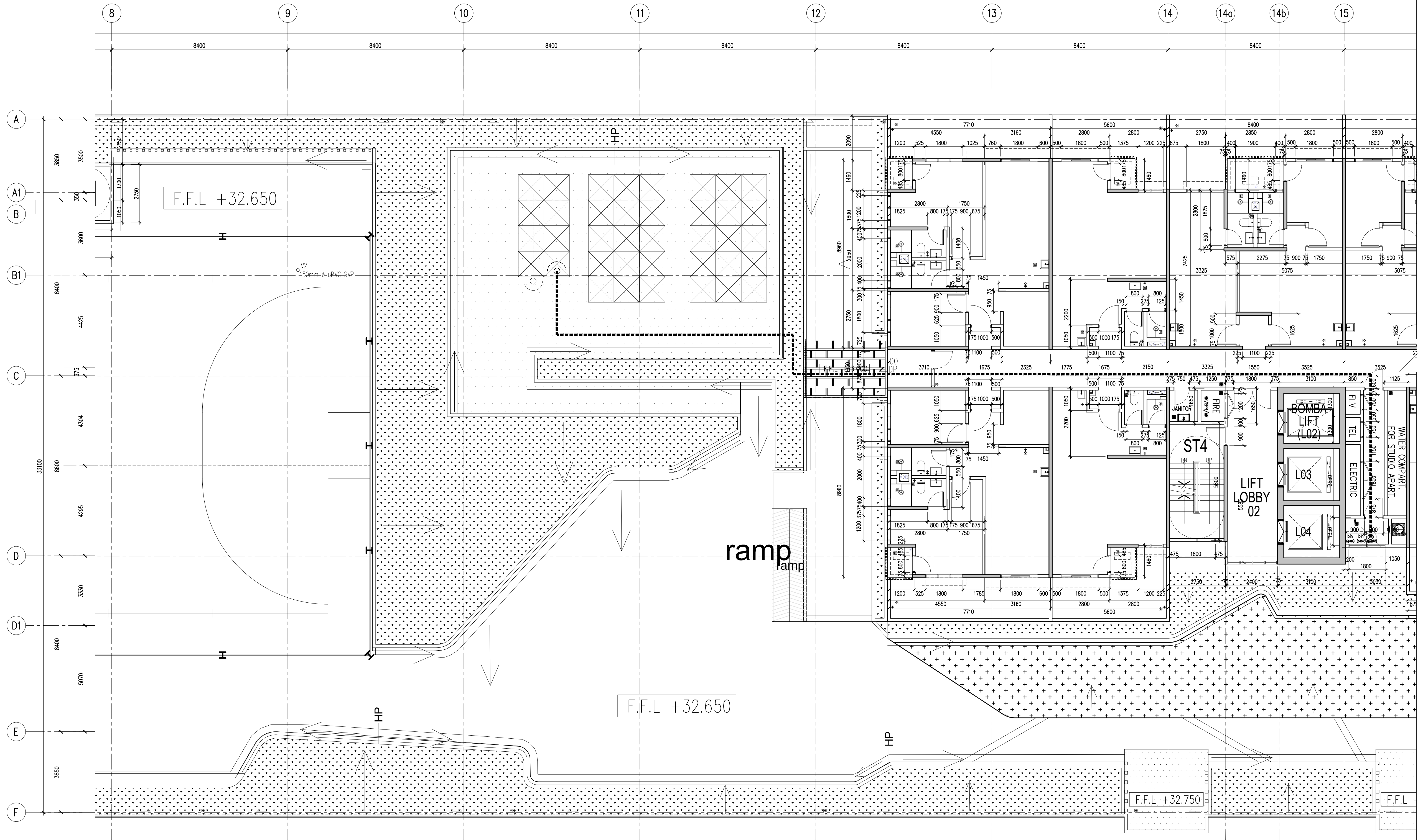
01 WALL SETTING OUT-LEVEL 9 ( PART 2 OF 7 ) 873-02 SCALE = 1 : 100
