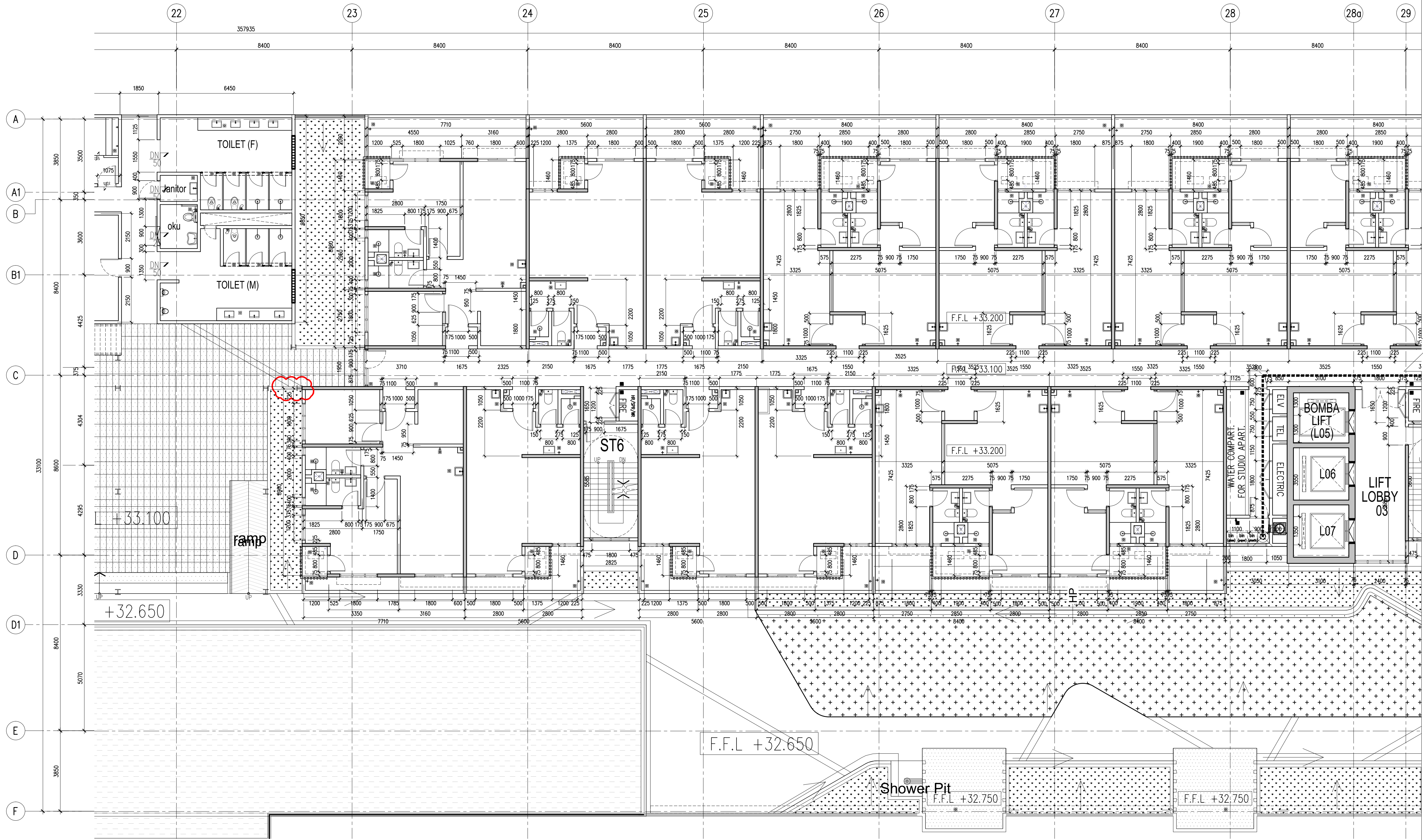
01 WALL SETTING OUT-LEVEL 9 ( PART 4 OF 7 ) 873-04 SCALE = 1 : 100
