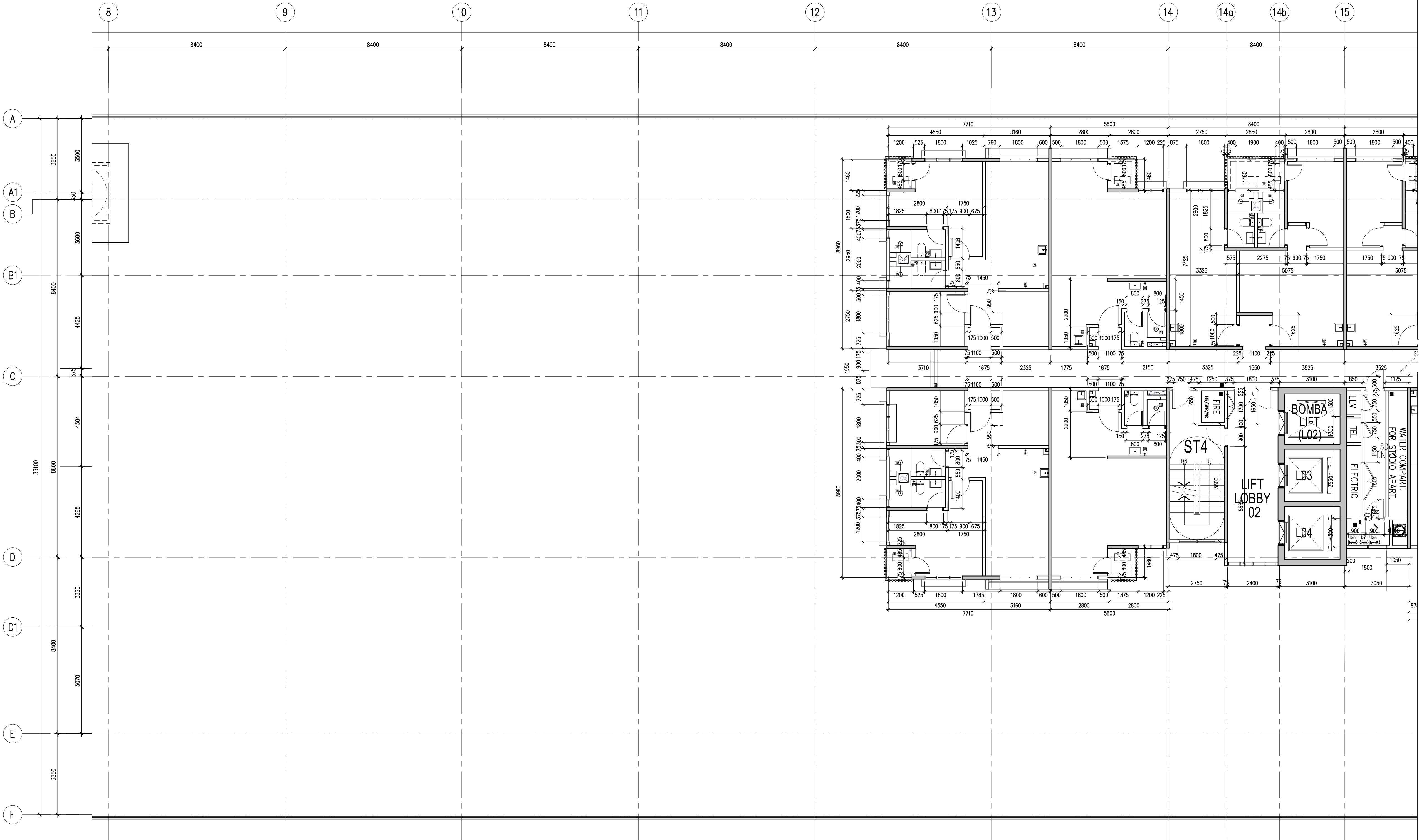
01 WALL SETTING OUT-LEVEL 10 ( PART 1 OF 4 ) 874-01 SCALE = 1 : 100
