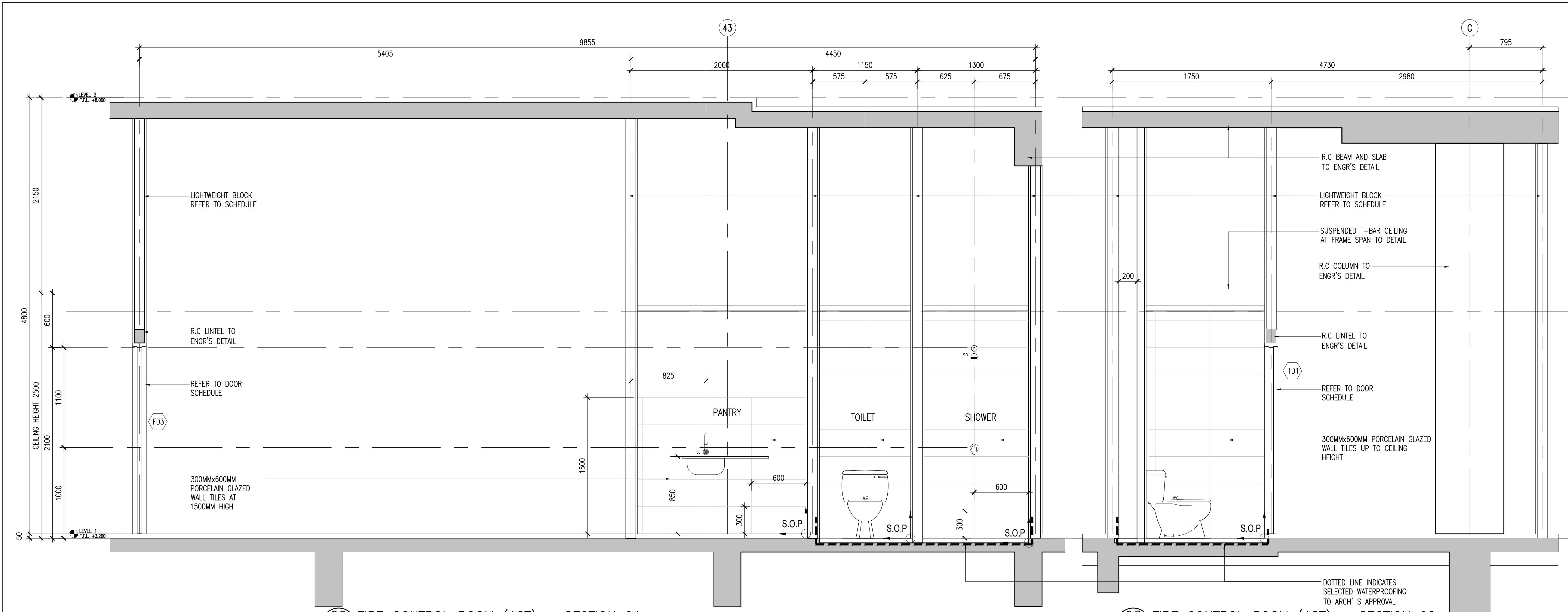
02 FIRE CONTROL ROOM (1ST) - SECTION 01 340-01 SCALE = 1 : 25
