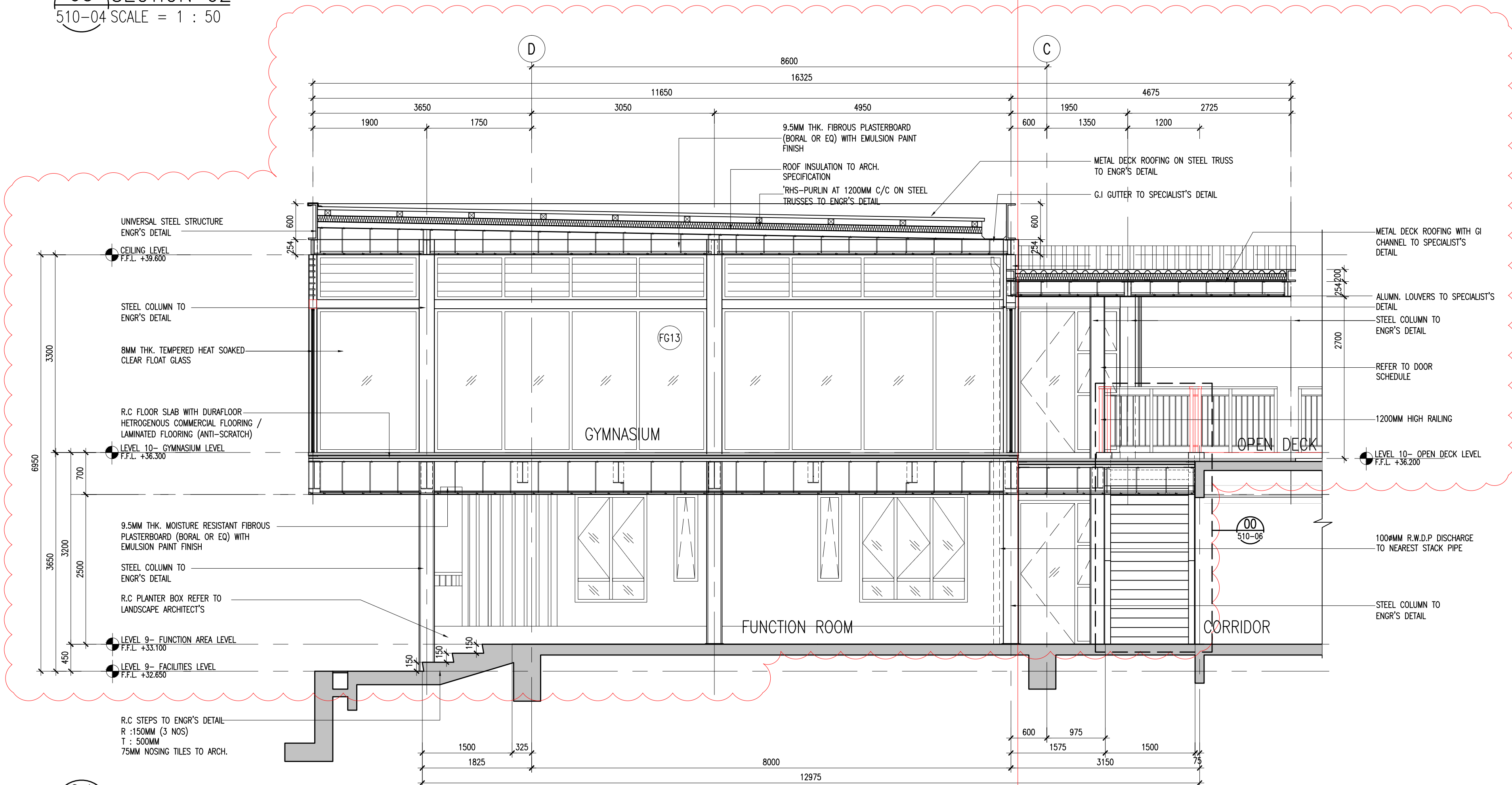
04 SECTION 01 510-04 SCALE = 1 : 50
