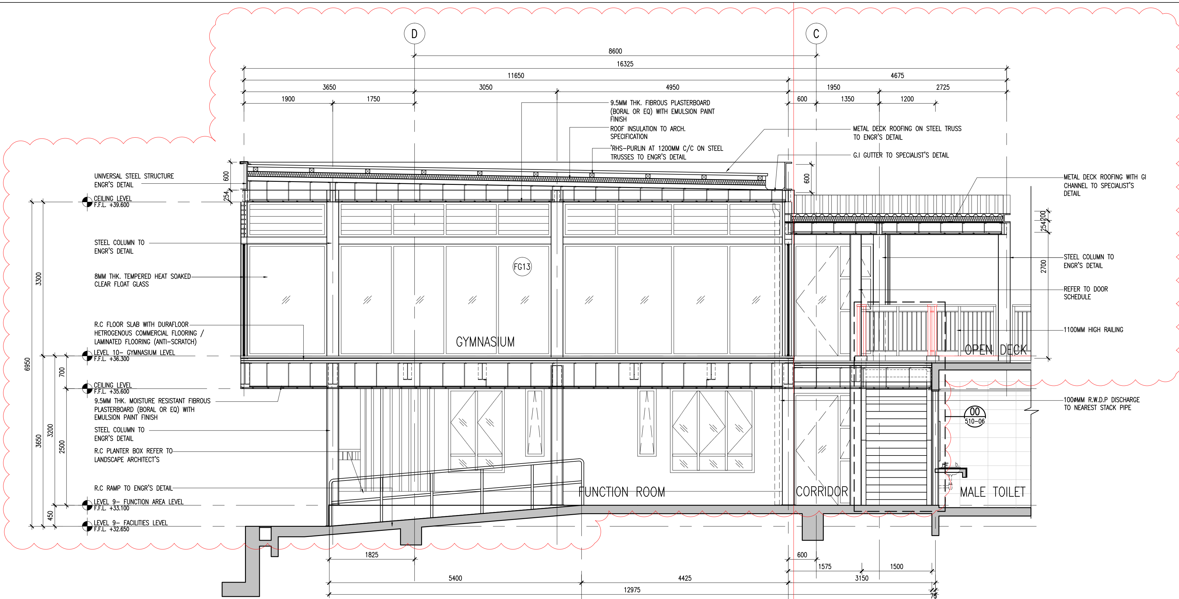
05 SECTION 02 510-04 SCALE = 1 : 50
