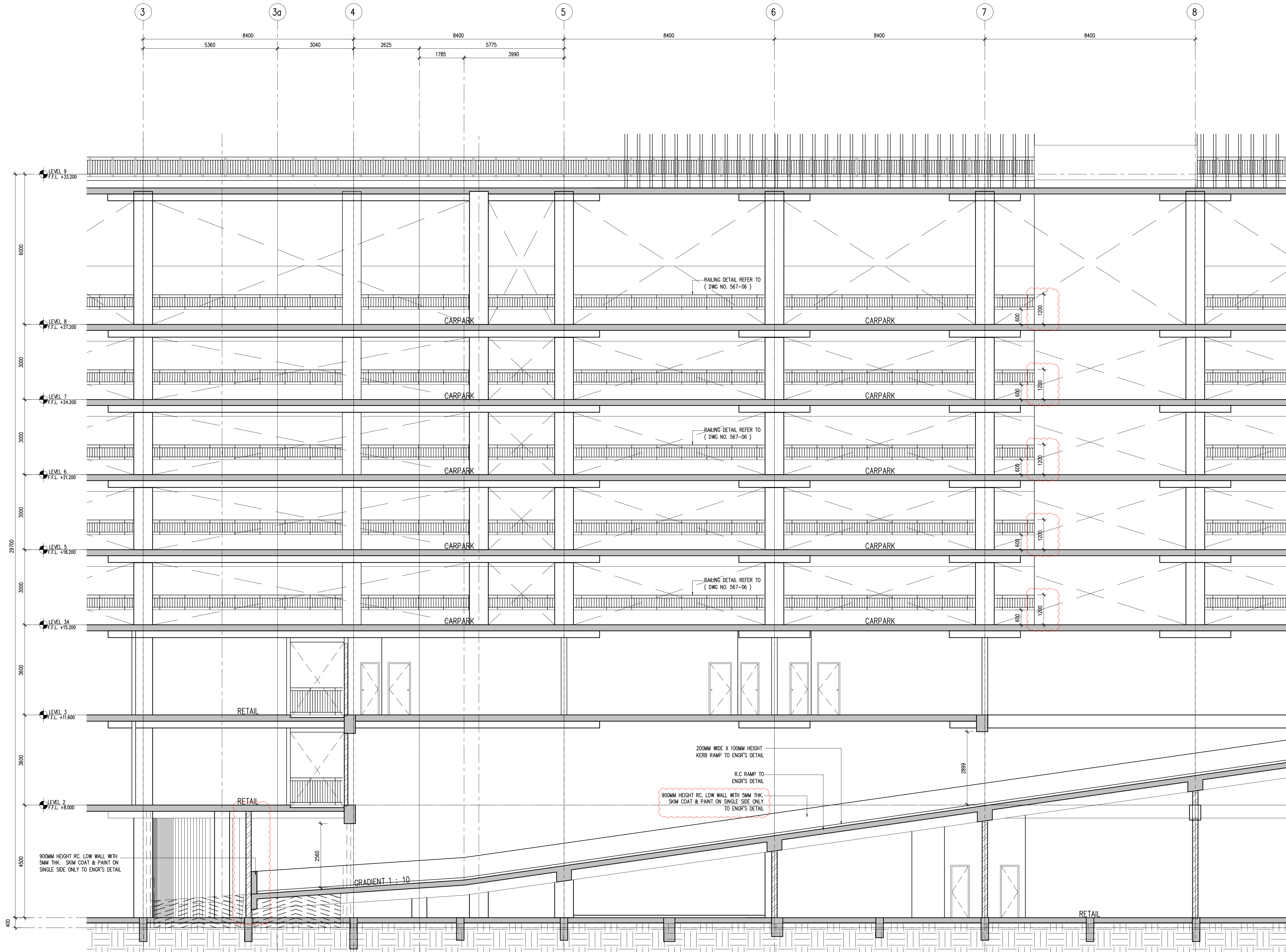
SECTION (1 OF 2) 523-04 SCALE = 1 : 75
