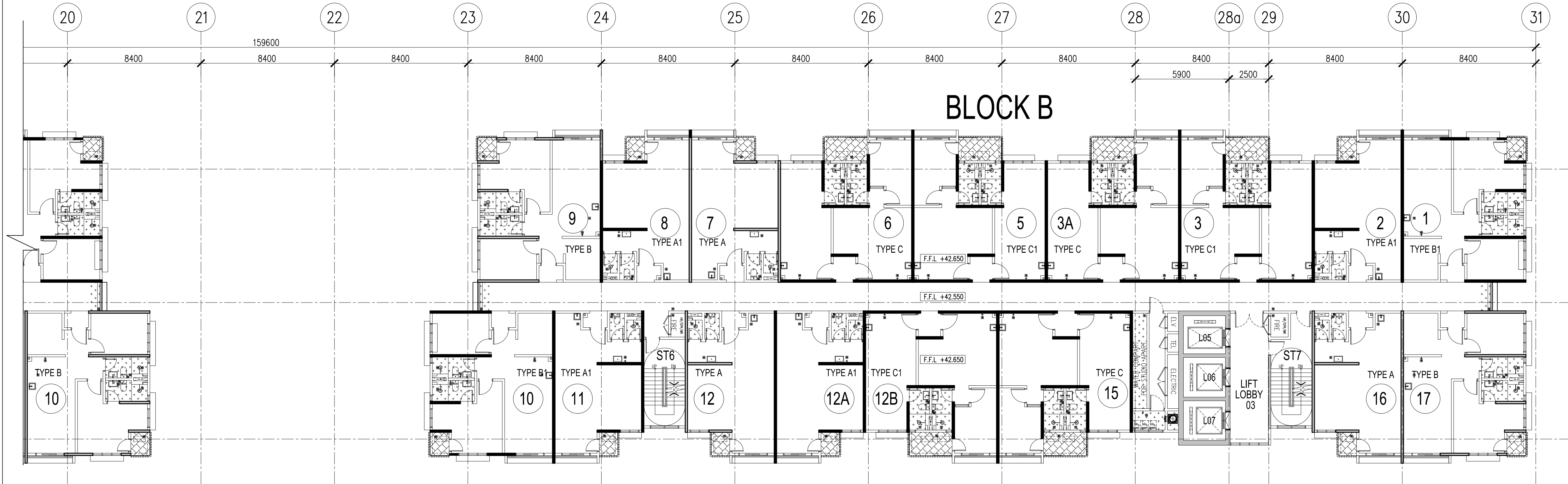
12 WATER PROOFING PLAN DEMARCATION (2 OF 2) – LEVEL 12–26 100 SCALE = 1 : 150
