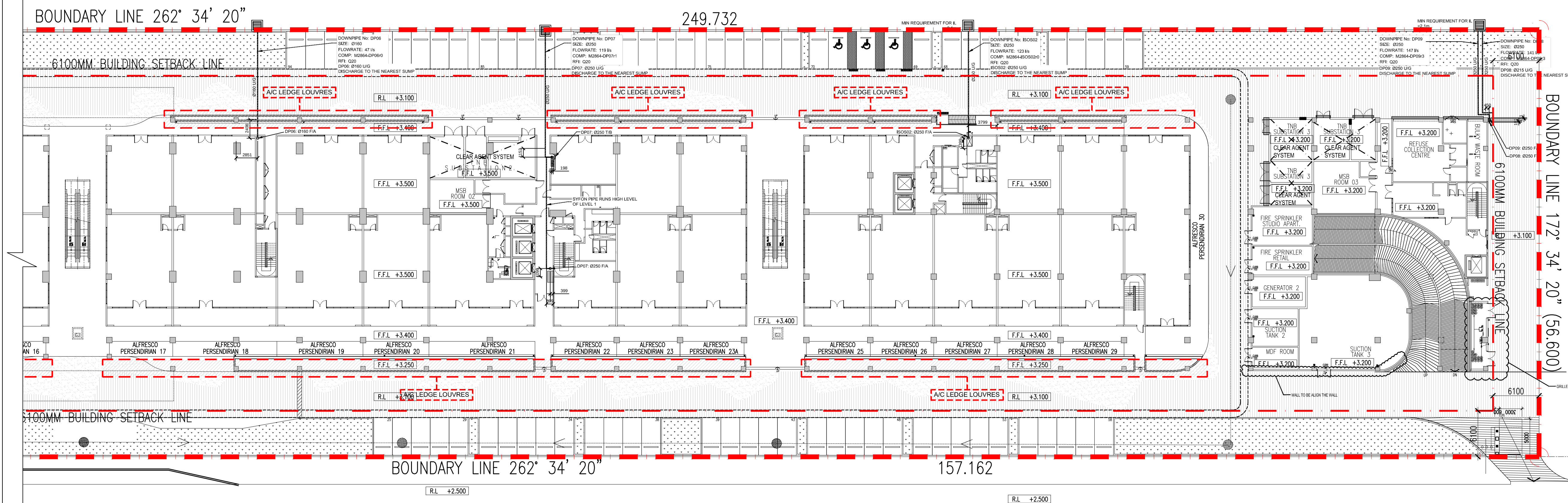
01 A/C LEDGE LOUVRES DETAIL - LOCATION PLAN LEV.1ST 536-01 NOT TO SCALE
