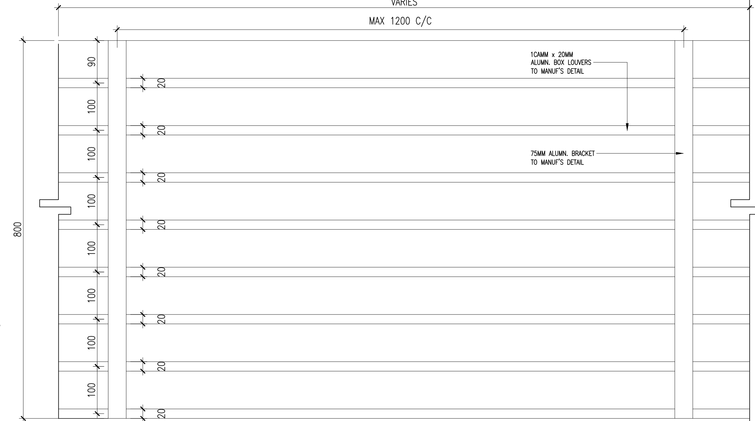
03 LOUVERS DETAIL - FRONT VIEW 536-03 SCALE = 1 : 5
