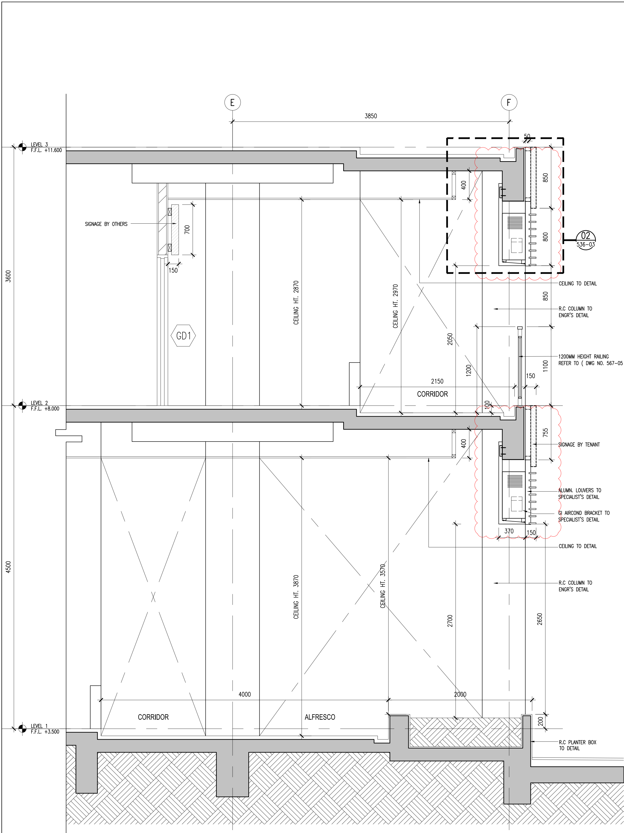
01 LOUVERS DETAIL - SECTION 536-03 SCALE = 1 : 25
