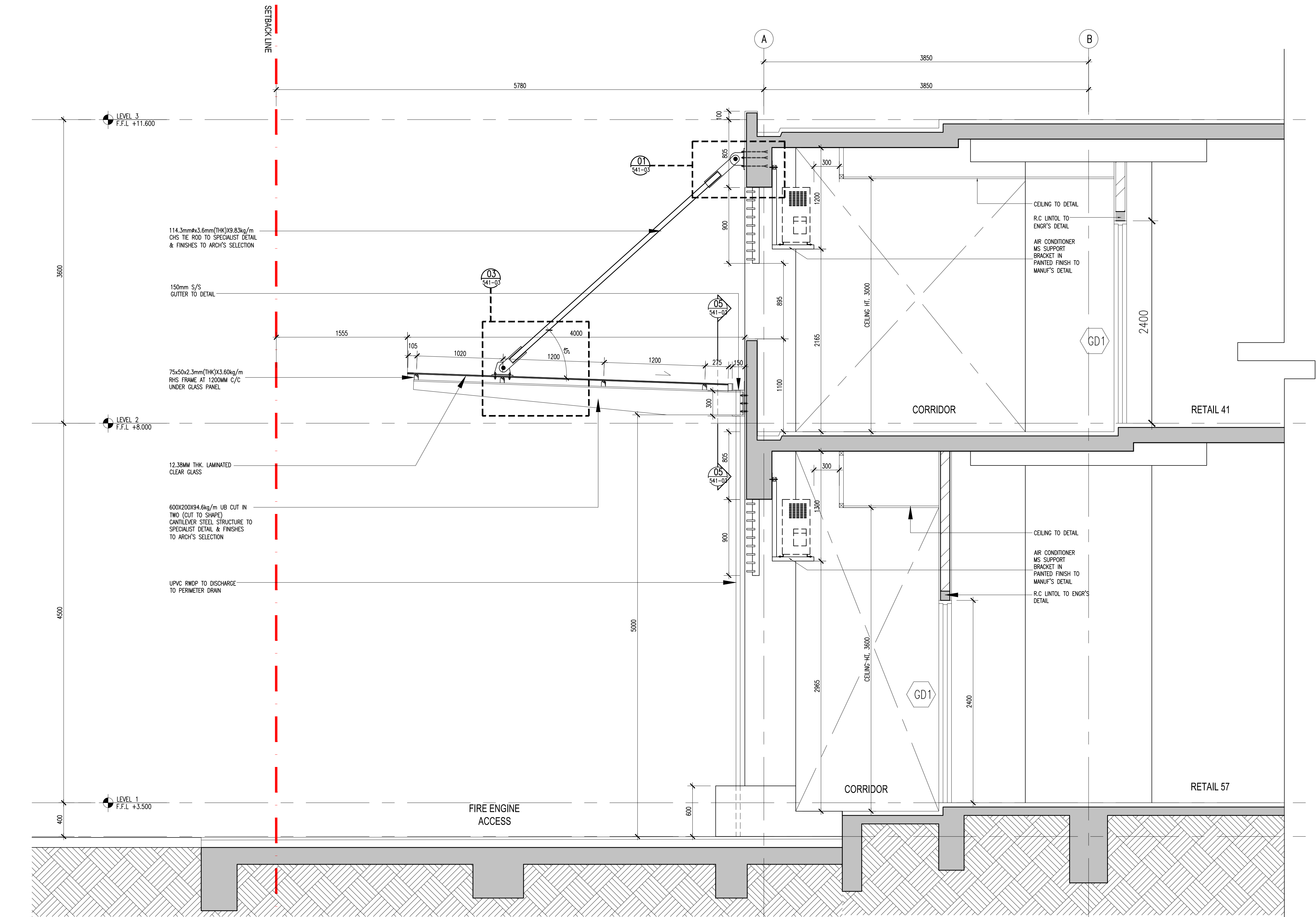
02 ENTRANCE GLASS CANOPY - PLAN 541 SCALE = 1 : 25
