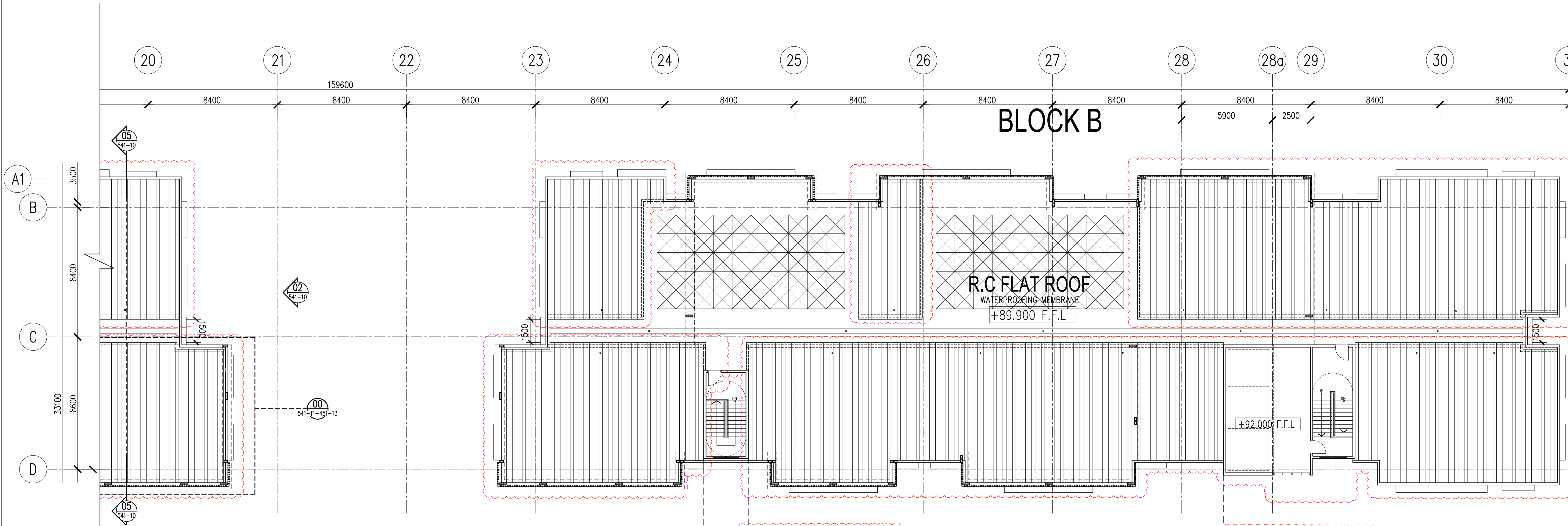
02 KEY PLAN - LOWER ROOF LEVEL (2 OF 2) 541-08 SCALE = 1 : 150
