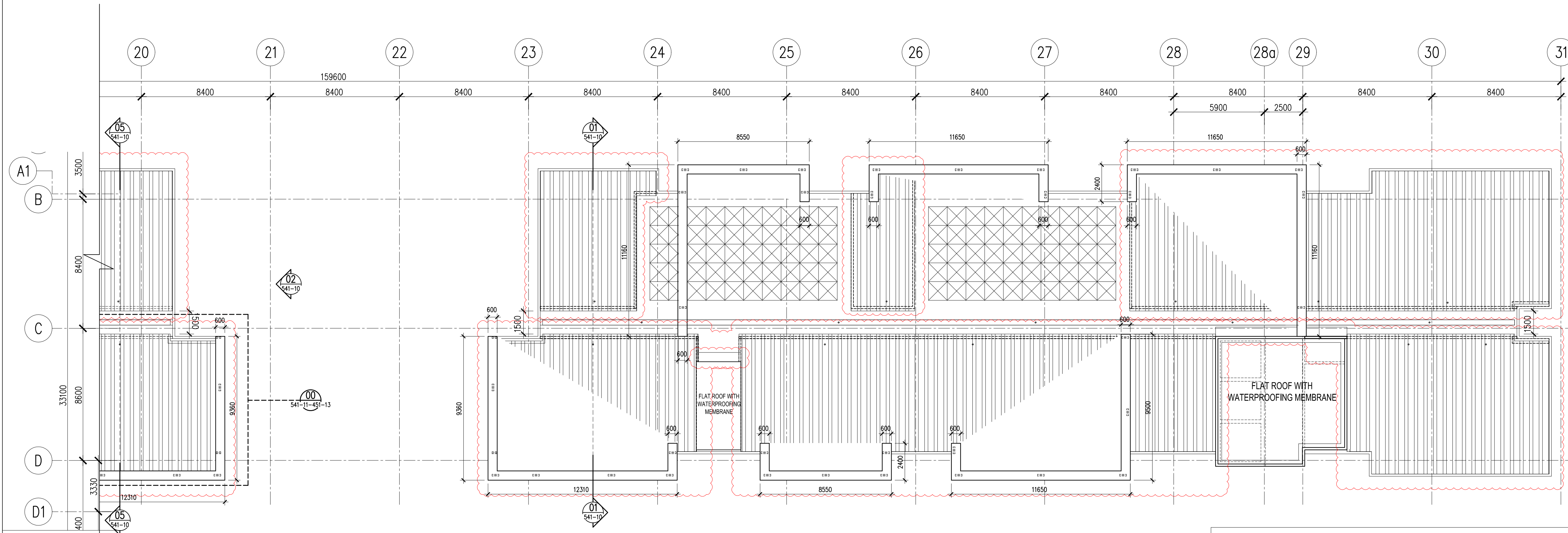
02 KEY PLAN – UPPER ROOF LEVEL (2 OF 2) 541-09 SCALE = 1 : 150
