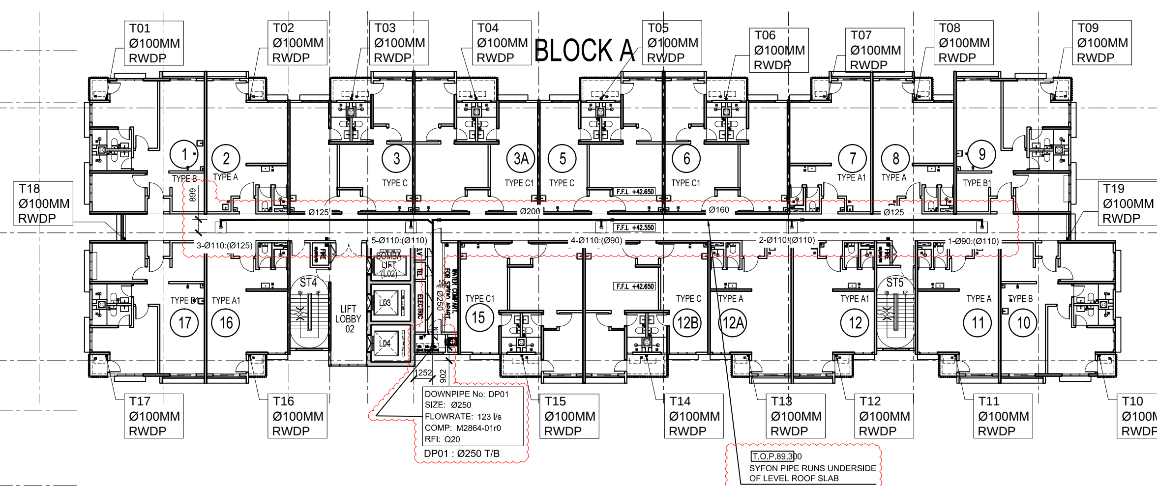
10 RAIN WATER DOWN PIPE – 26TH. FLOOR PLAN 543 SCALE = 1 : 250
