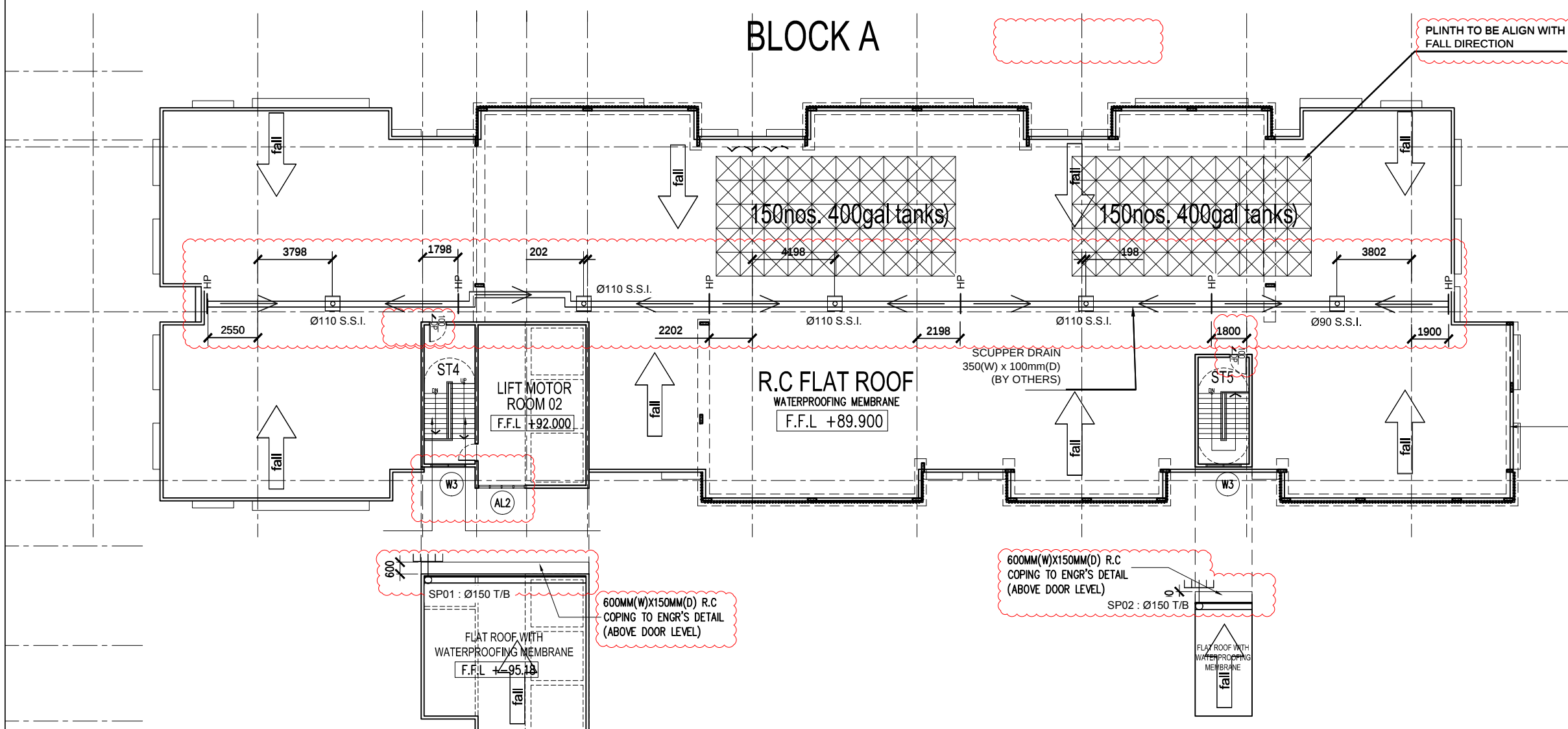
12 RAIN WATER DOWN PIPE – ROOF PLAN 543 SCALE = 1 : 250
