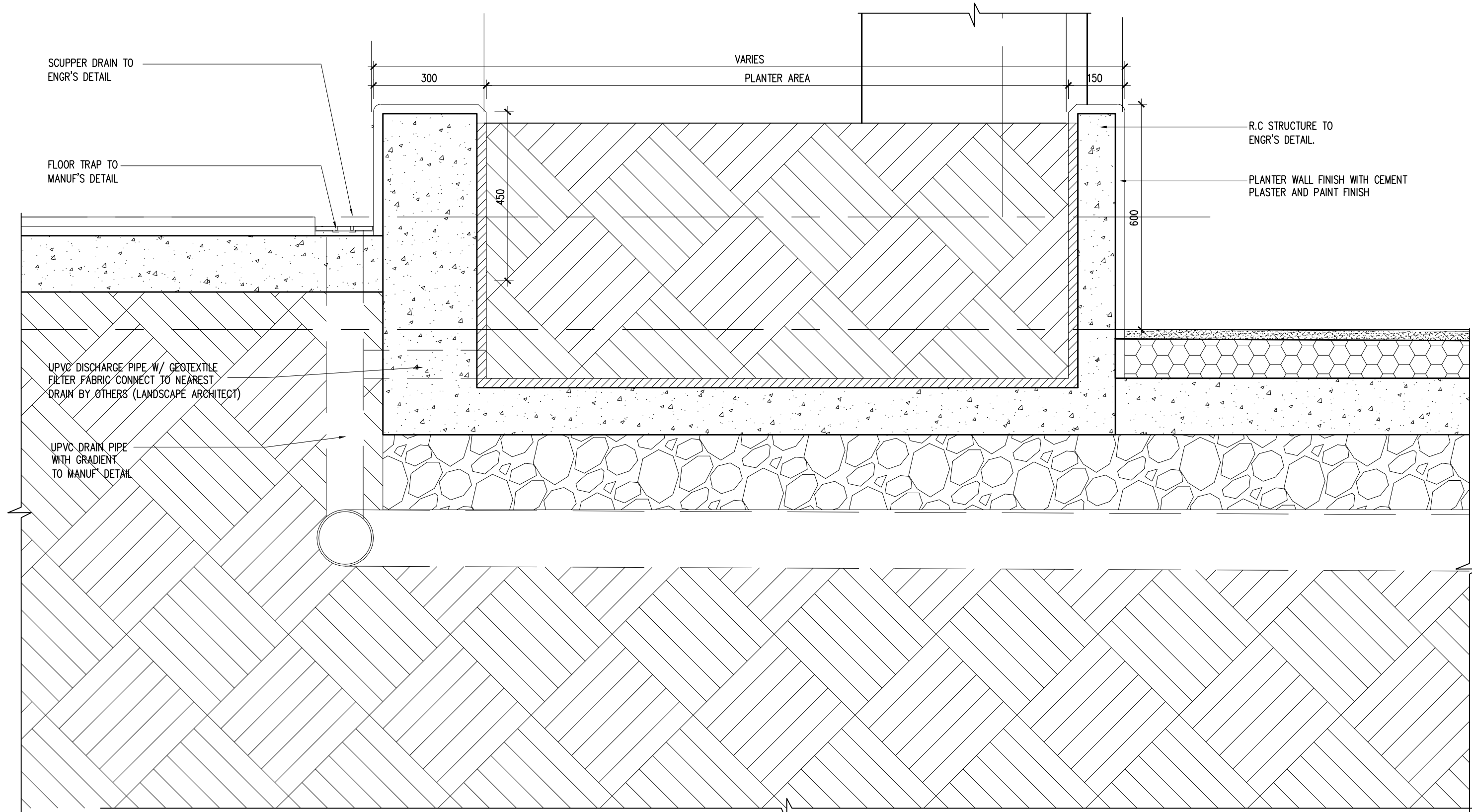
02 TYPICAL DETAIL SCALE = 1 : 5
