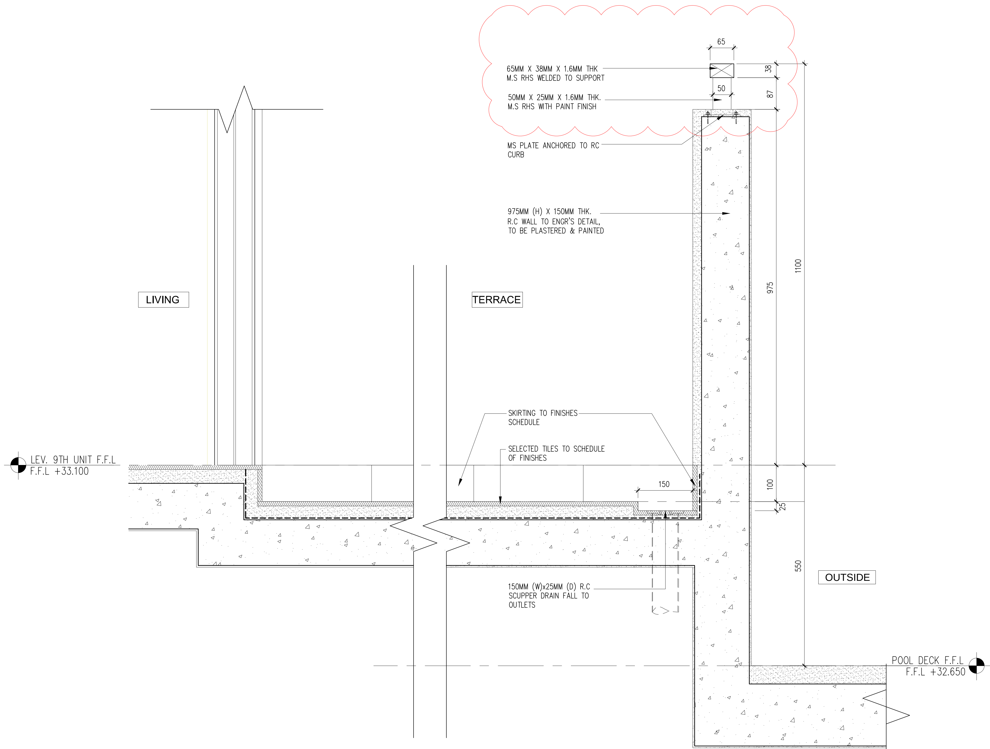
01 RAILING DETAIL AT TERRACE OF TYPICAL UNIT – SECTION 1 567-08 SCALE = 1 : 5
