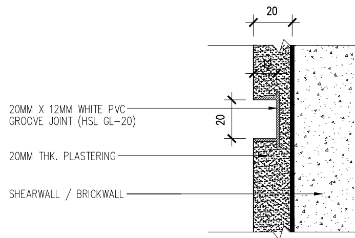
0.3 GROOVE JOINT DETAIL 610-01 SCALE = 1 : 2
