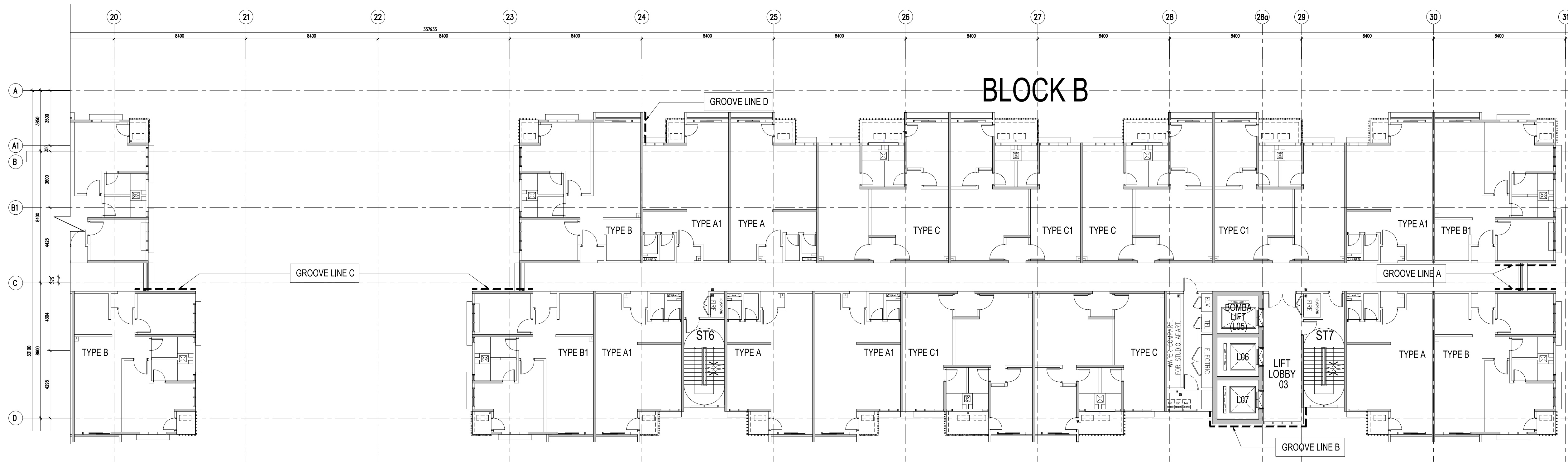
02 GROOVE LINE LOCATION AT TYPICAL UNIT PLAN 610-01 SCALE = 1 : 150
