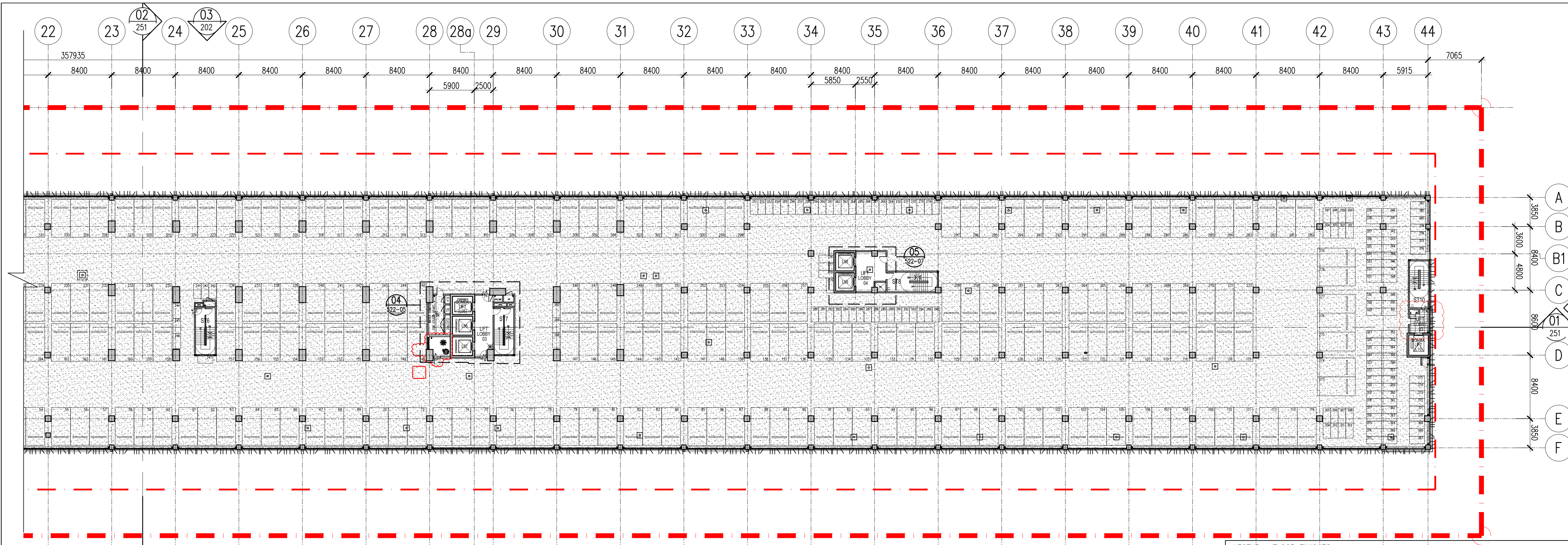
02 FLOOR FINISHES PLAN DEMARCATION (2 OF 2) - LEVEL 8 811-07 SCALE = 1 : 300
