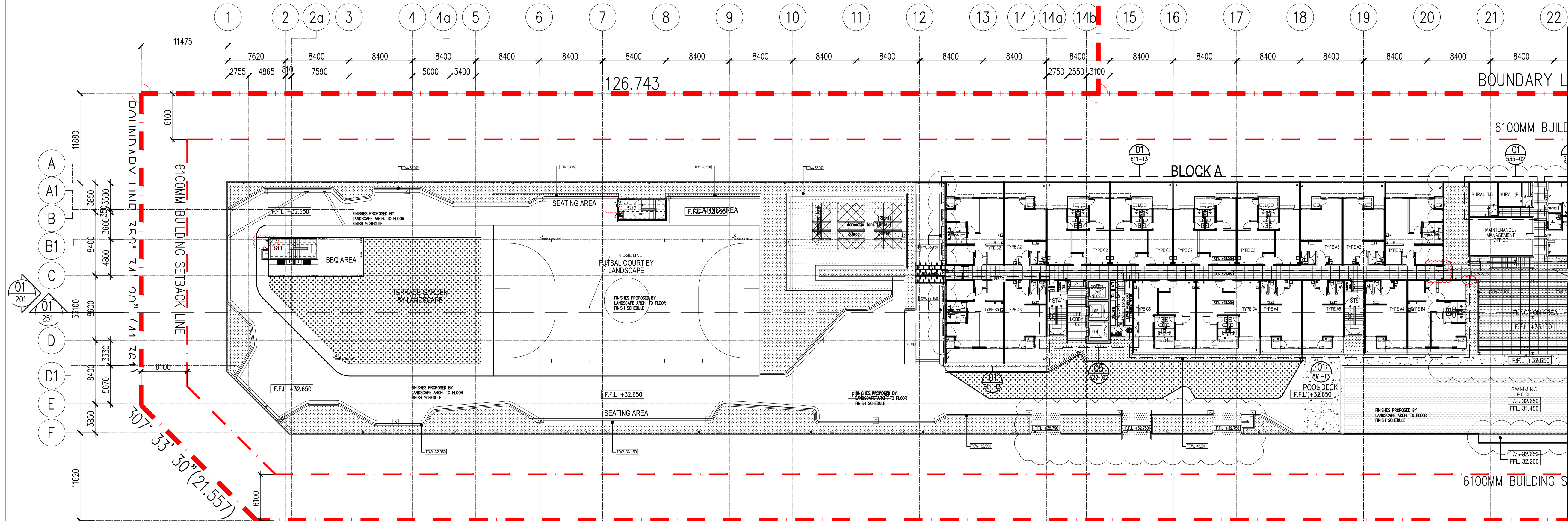
01 FLOOR FINISHES PLAN DEMARCATION (1 OF 2) - LEVEL 9 811-08 SCALE = 1 : 300
