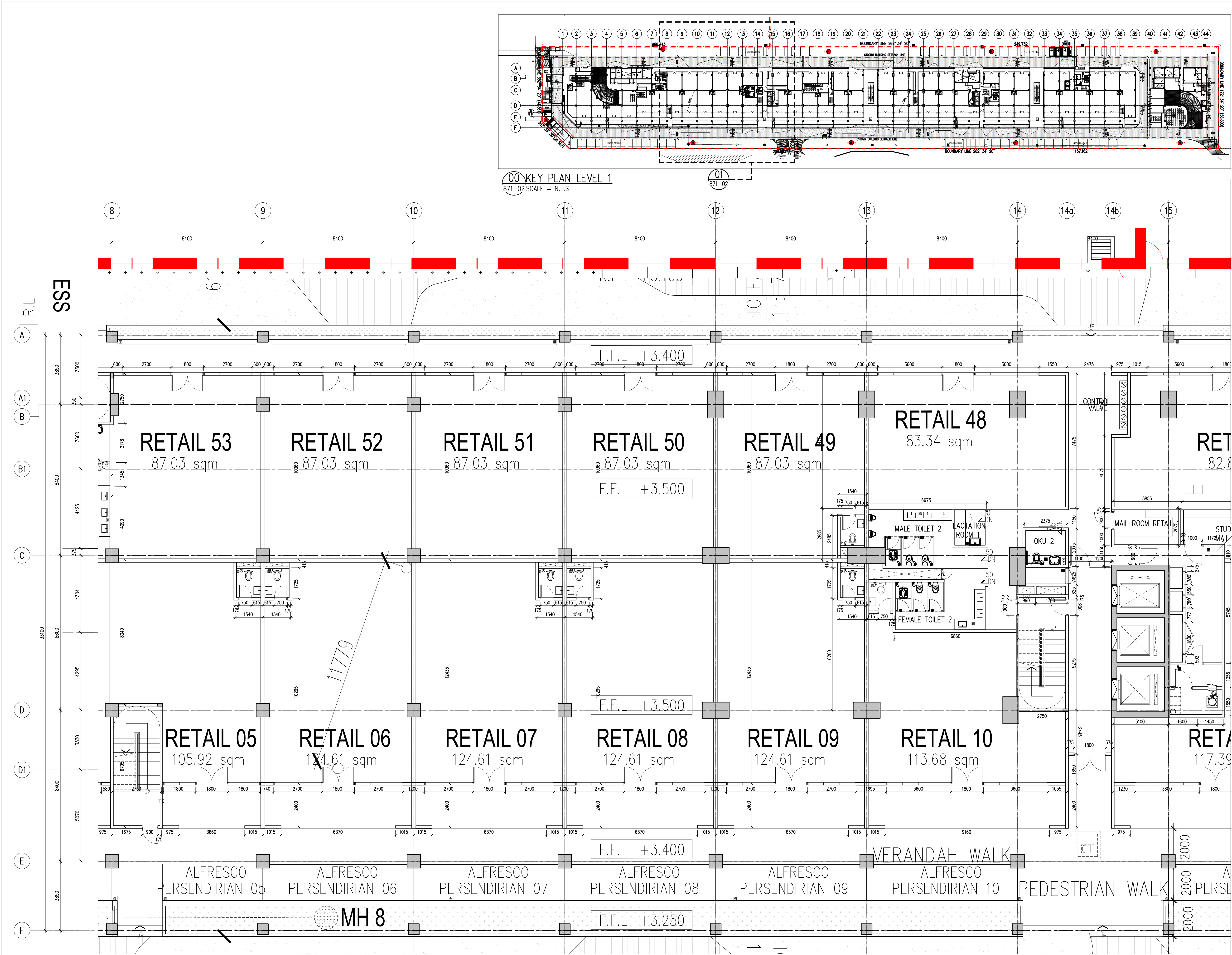
01 WALL SETTING OUT-LEVEL 1 PART 2 871-02 SCALE = 1 : 100
