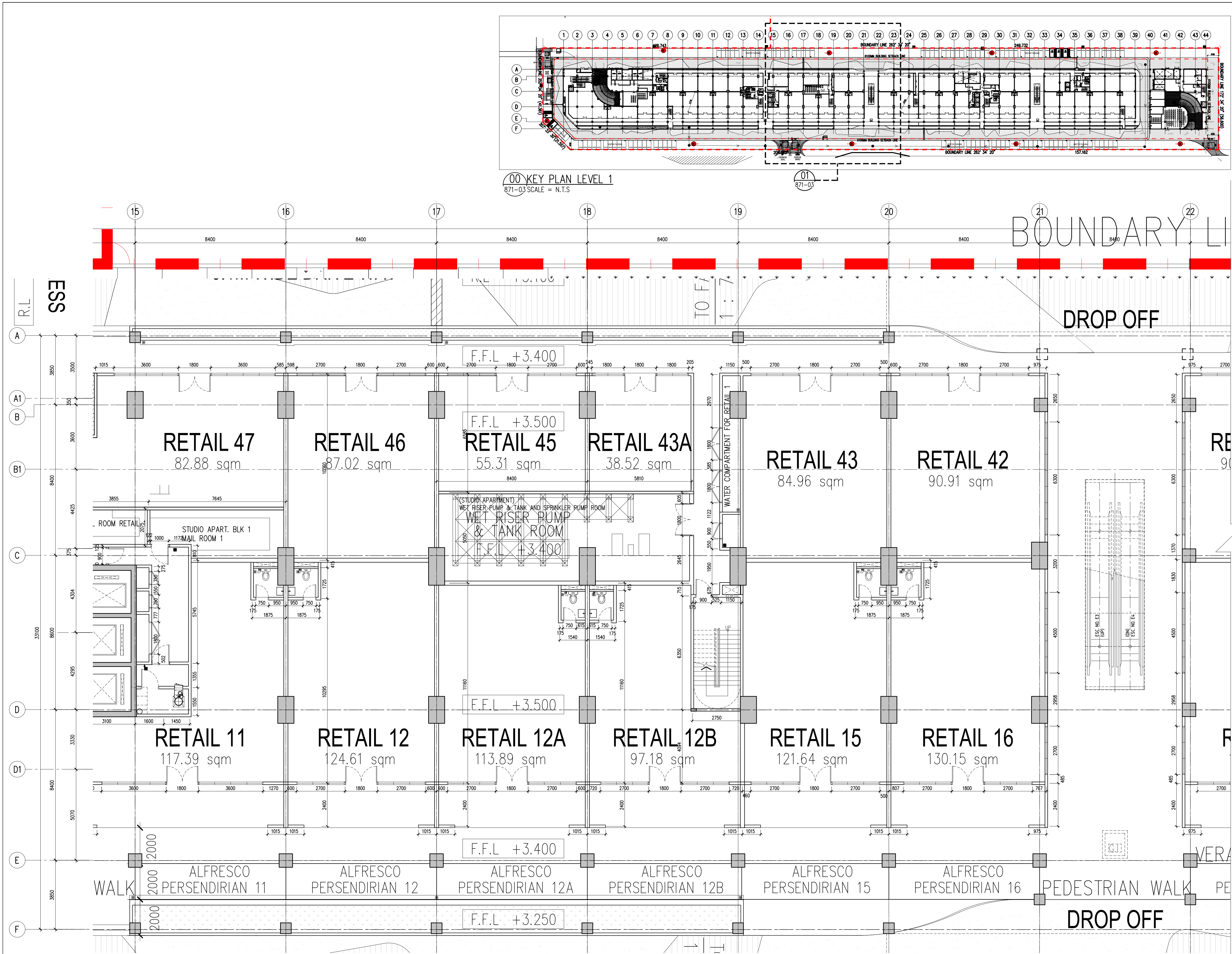
01 WALL SETTING OUT-LEVEL 1 PART 3 871-03 SCALE = 1 : 100
