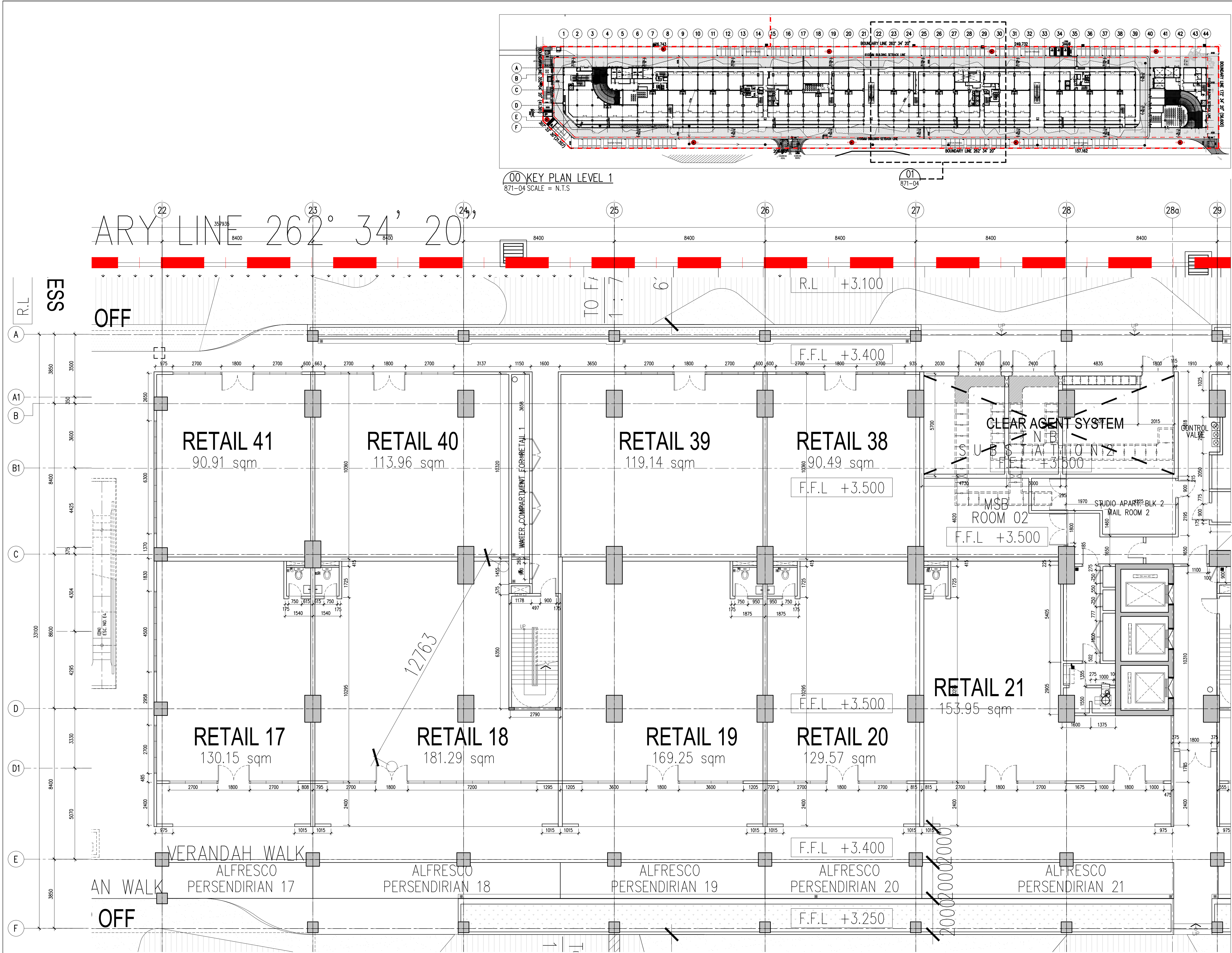
01 WALL SETTING OUT-LEVEL 1 PART 4 871-04 SCALE = 1 : 100
