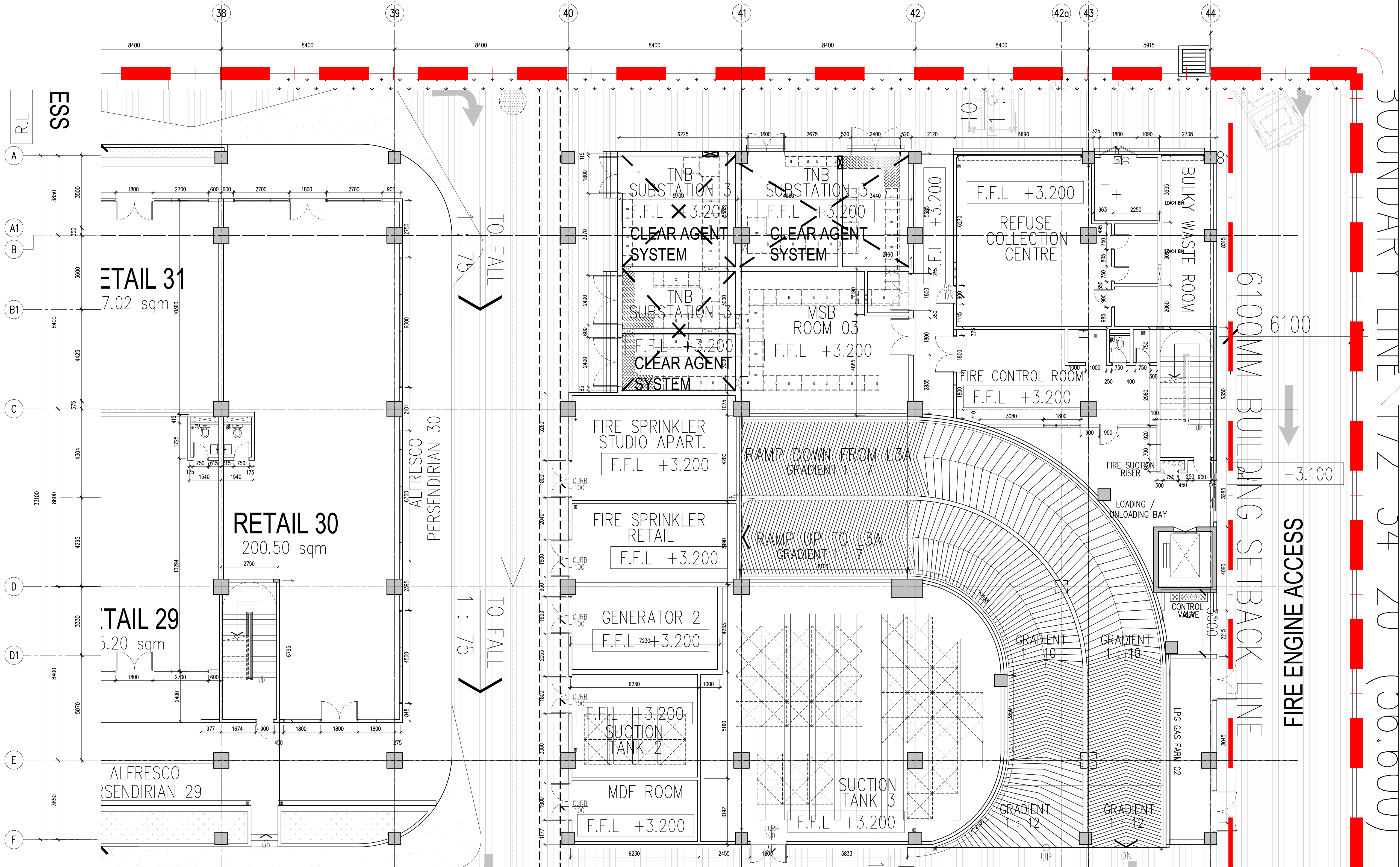
01 WALL SETTING OUT-LEVEL 1 PART 7 871-07 SCALE = 1 : 100
