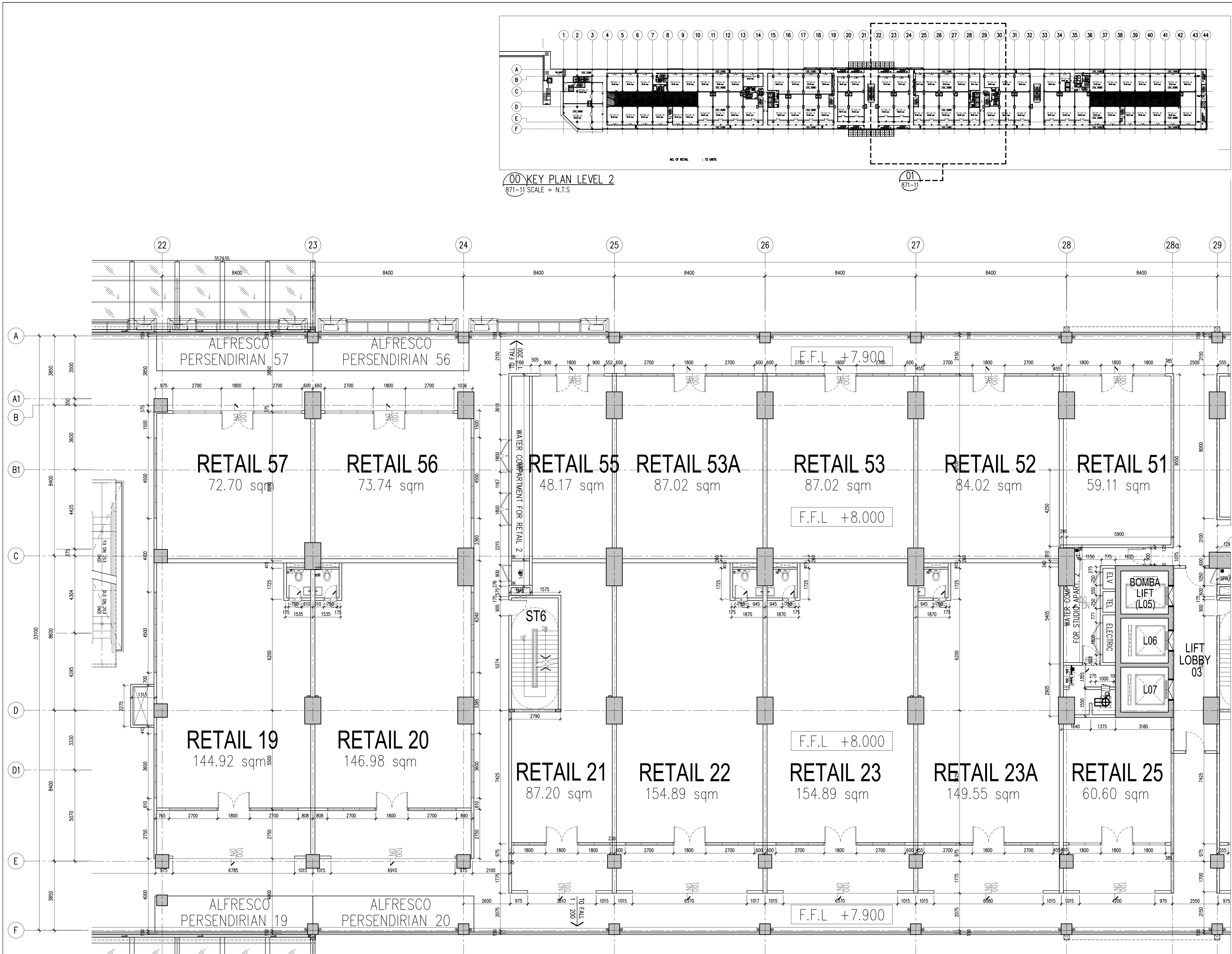
01 WALL SETTING OUT-LEVEL 2 PART 4 871-11 SCALE = 1 : 100
