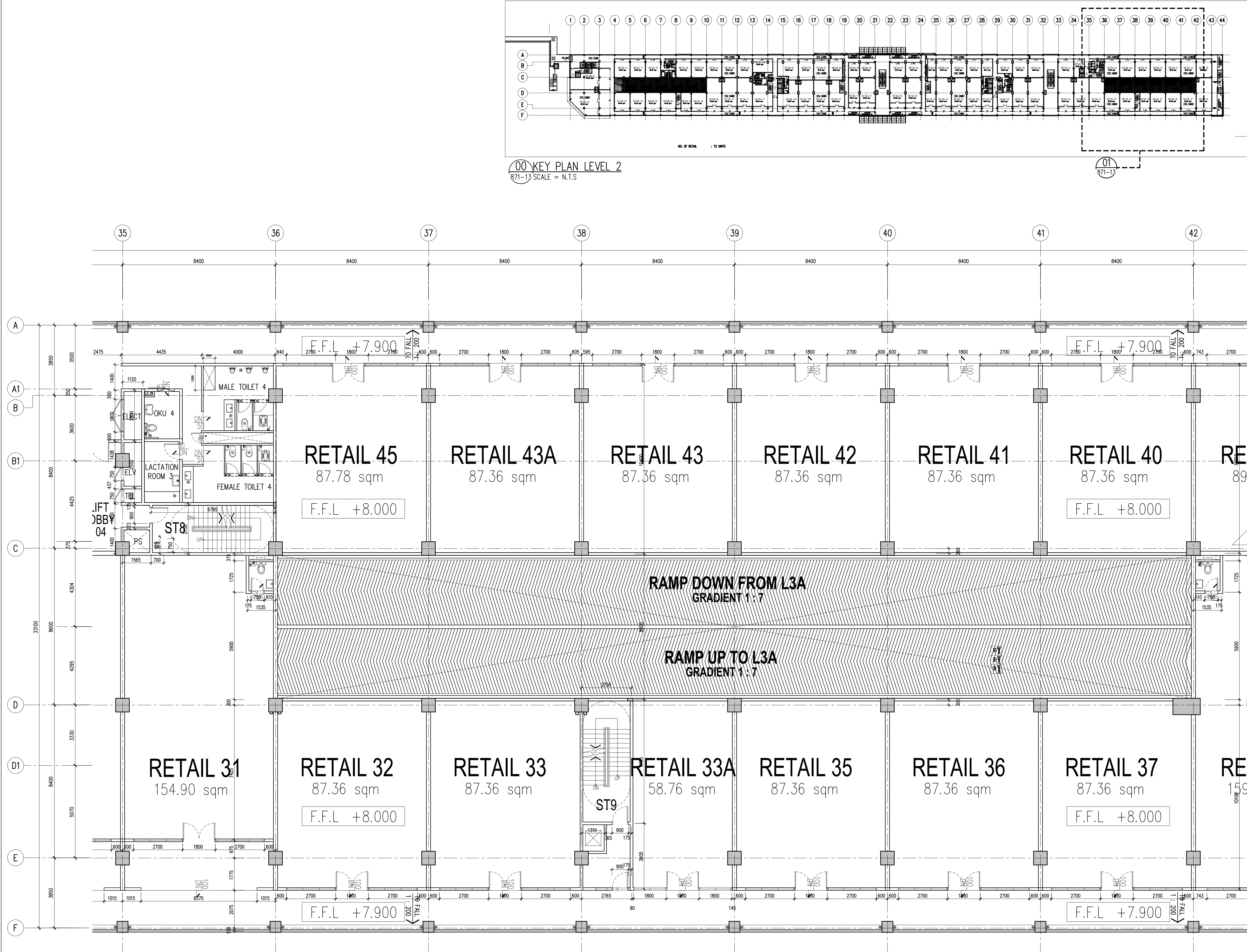
01 WALL SETTING OUT-LEVEL 2 PART 6 871-13 SCALE = 1 : 100
