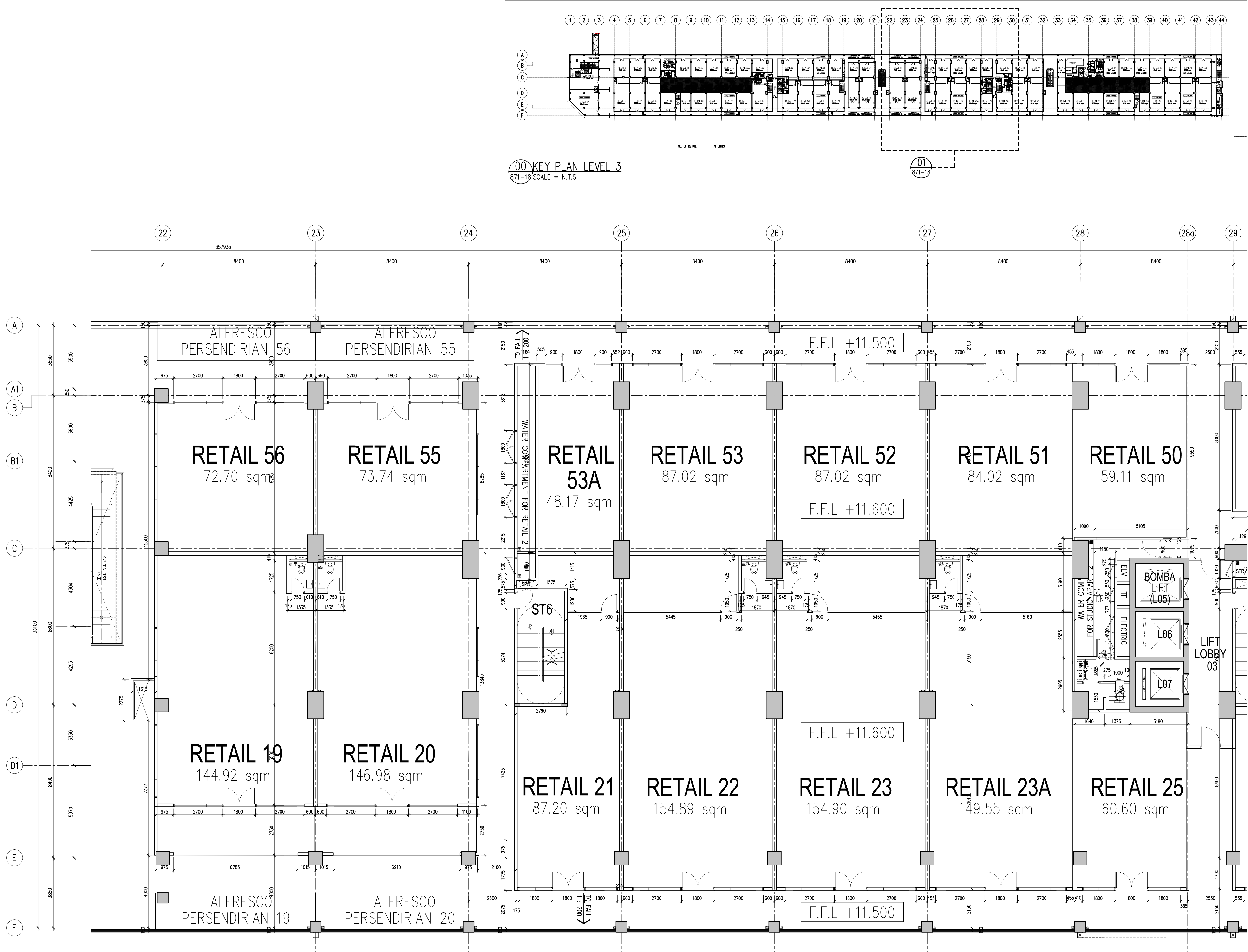
01 WALL SETTING OUT-LEVEL 3 PART 4 871-18 SCALE = 1 : 100
