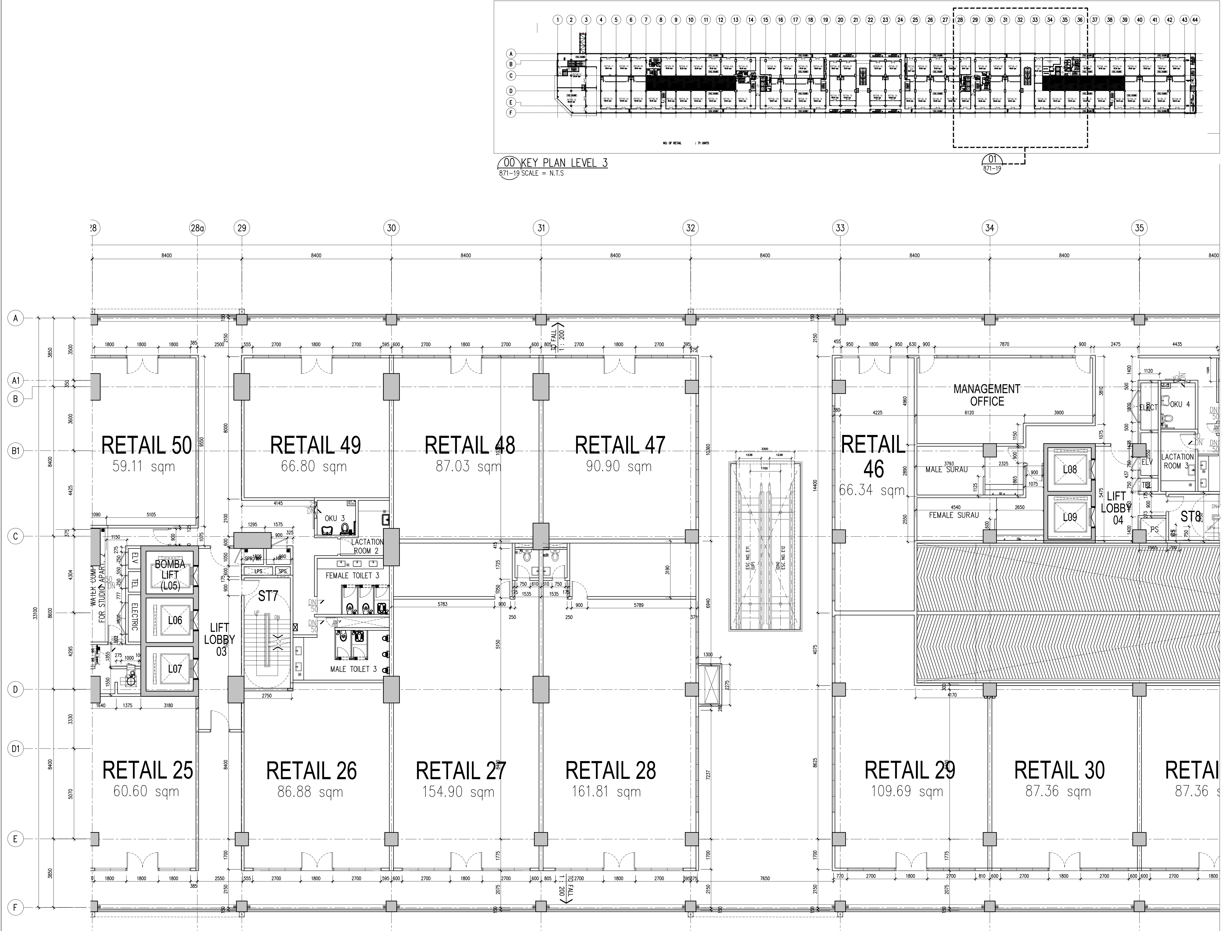
01 WALL SETTING OUT-LEVEL 3 PART 5 871-19 SCALE = 1 : 100
