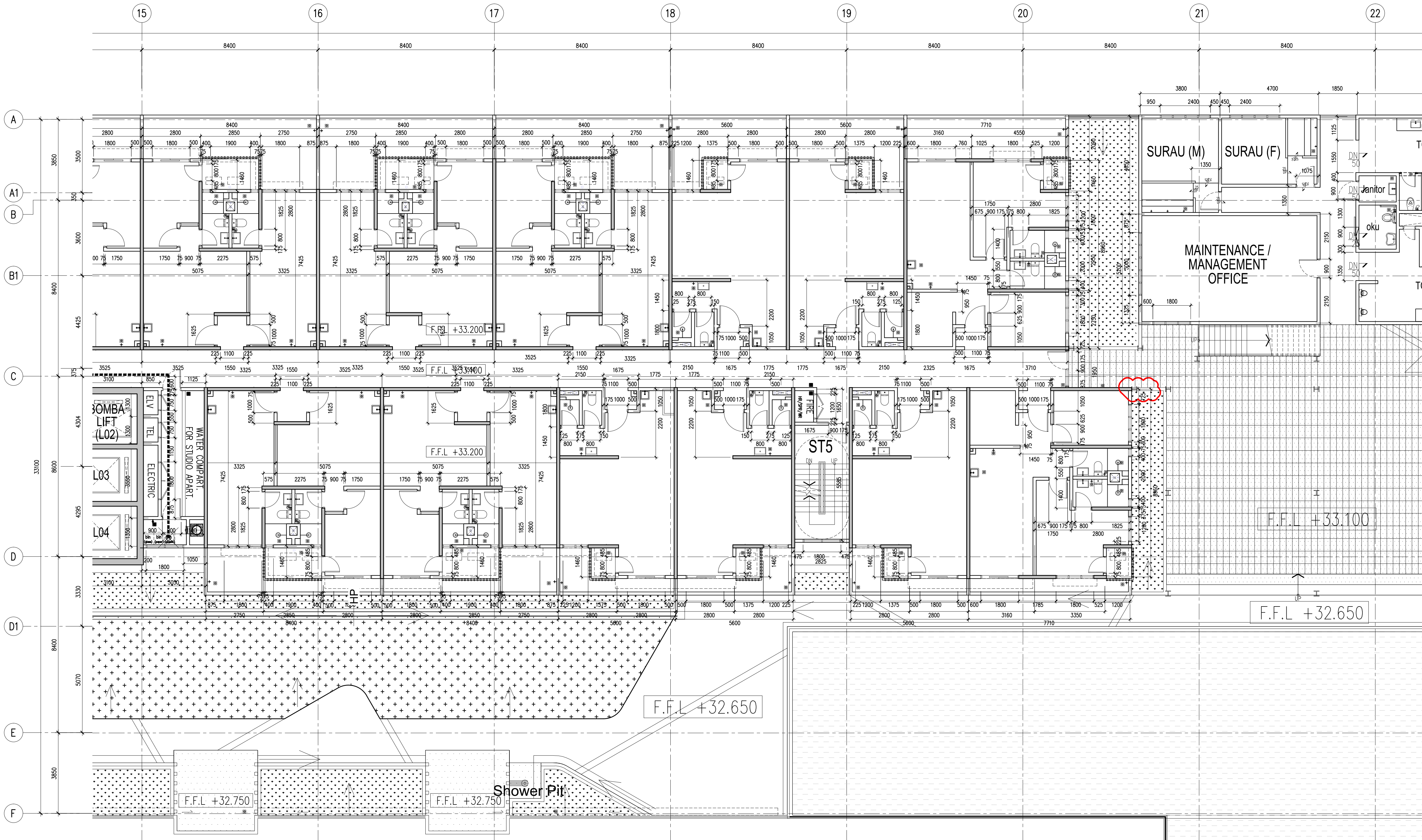
01 WALL SETTING OUT-LEVEL 9 ( PART 3 OF 7 ) 873-03 SCALE = 1:100
