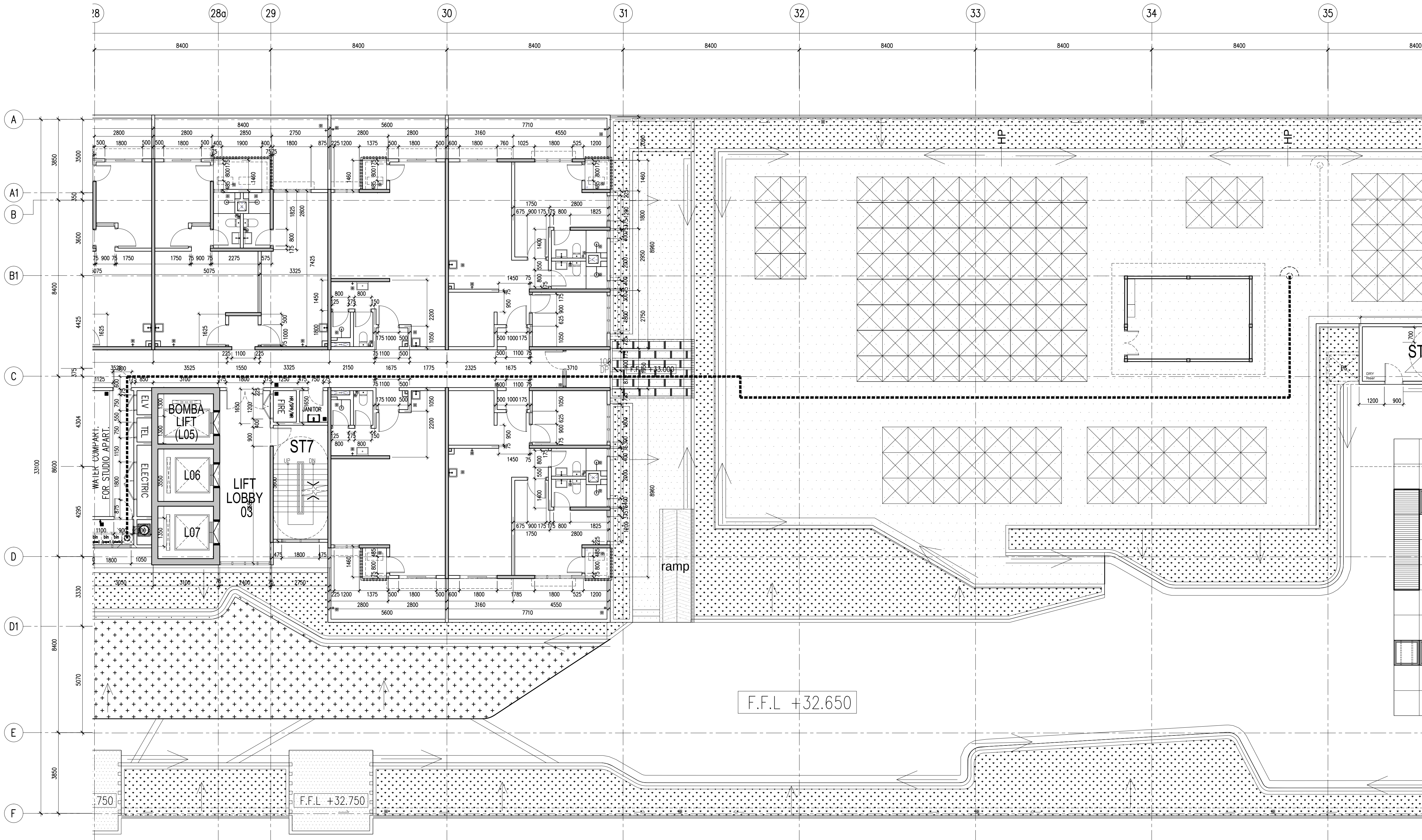
01 WALL SETTING OUT-LEVEL 9 ( PART 5 OF 7 ) 873-05 SCALE = 1 : 100
