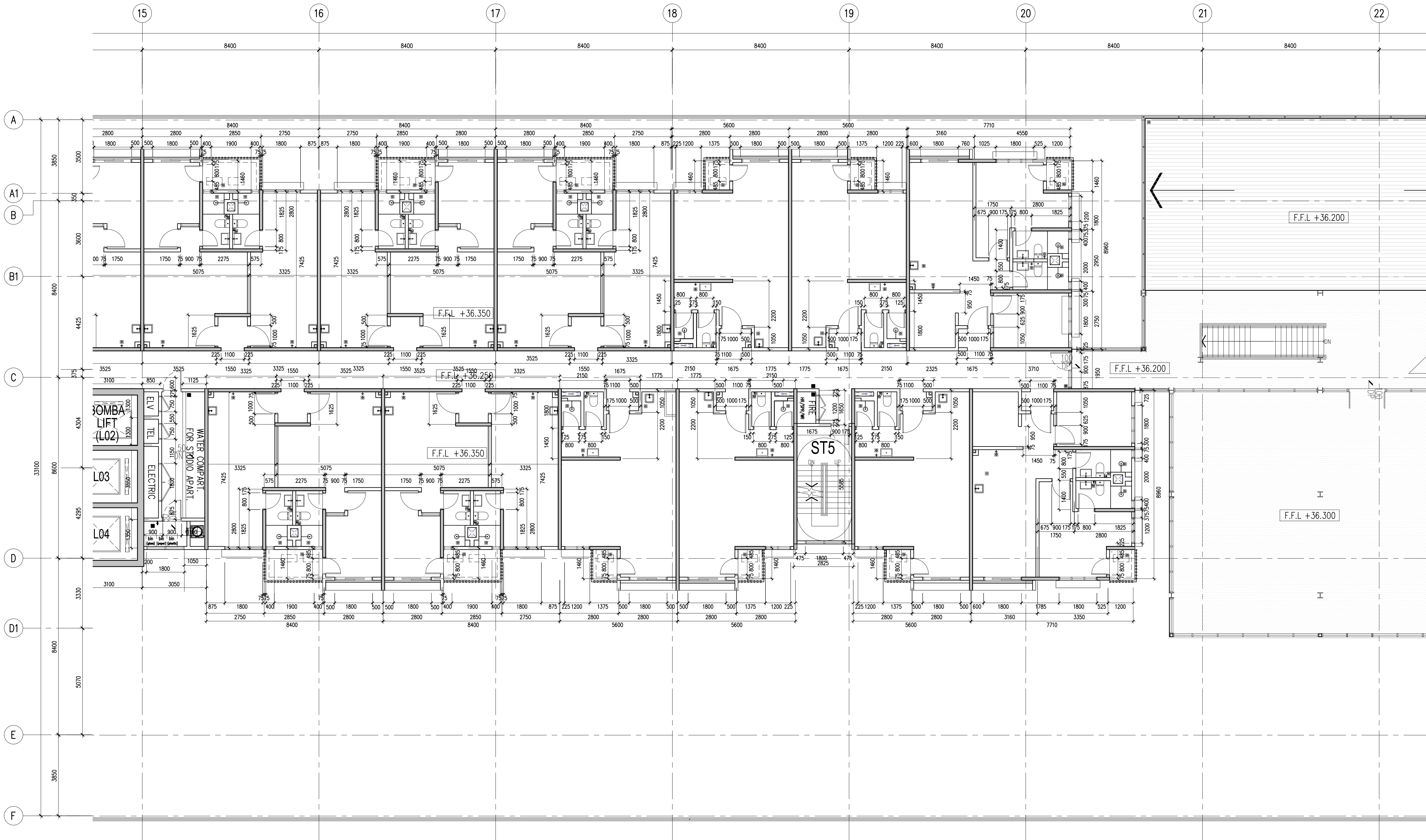
01 WALL SETTING OUT-LEVEL 10 (PART 2 OF 4 ) 874-02 SCALE = 1 : 100
