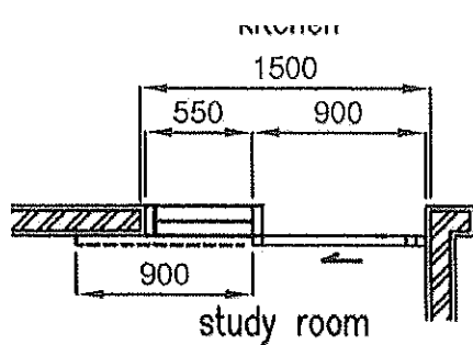
study room internal typical plan view
