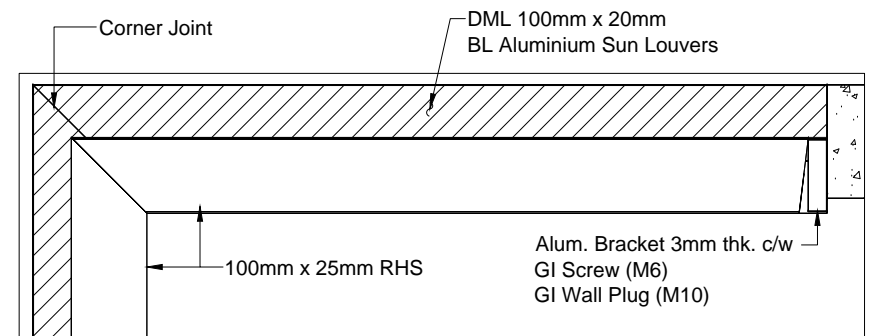
Enlarge View 1 Scale : 1/20
