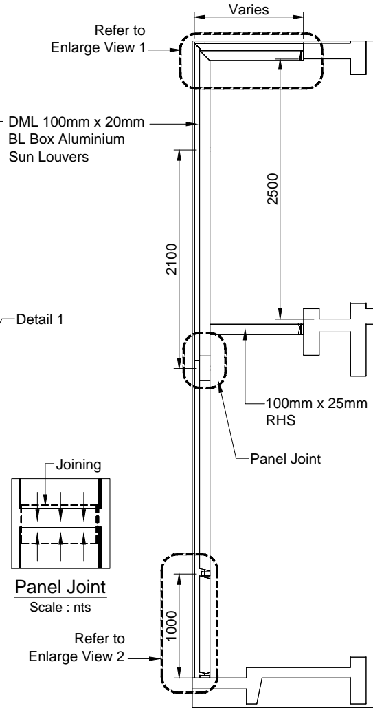
Typical Section View Scale : 1/50
