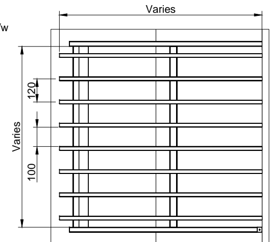
Typical Plan View Scale : 1/20
