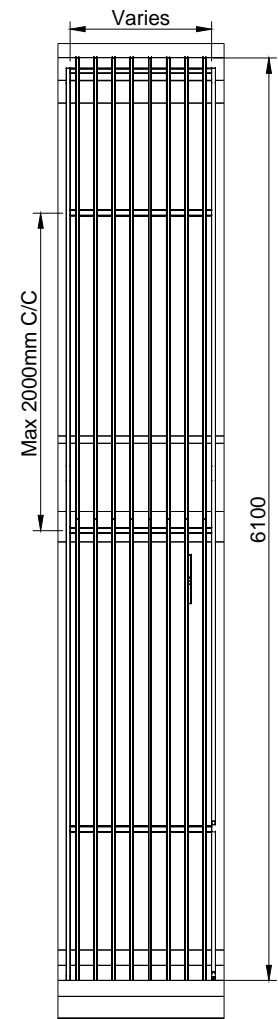
Typical Section View Scale : 1/50
