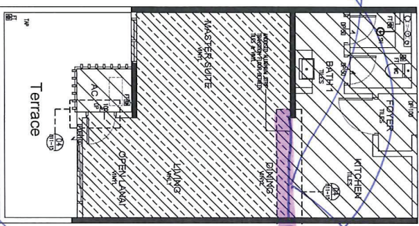
01 KEY PLAN TYPE A.A1&A2 251 SCALE = 1 : 50
