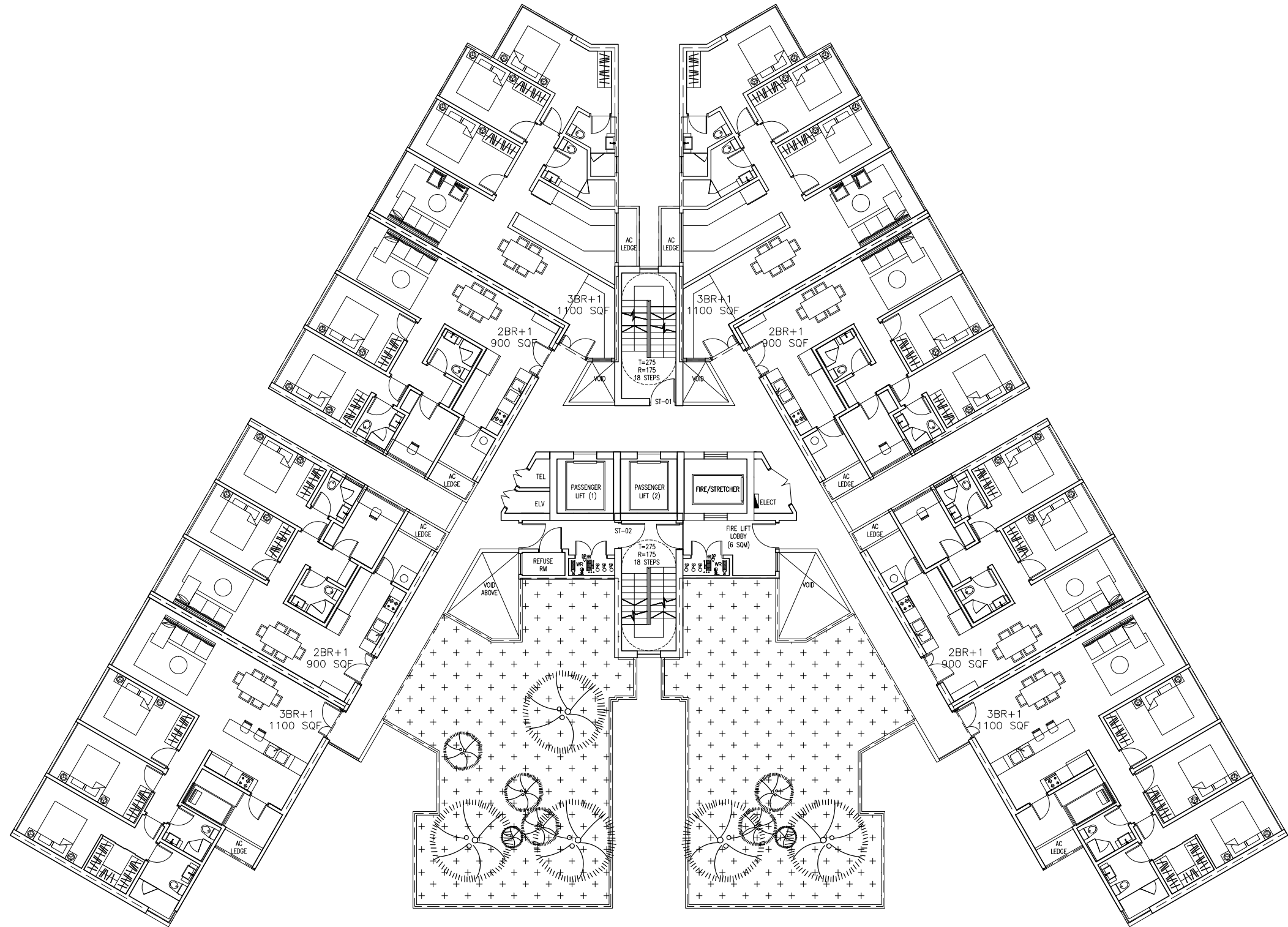
SERVICE APARTMENT_13TH FLOOR scale 1: 200
