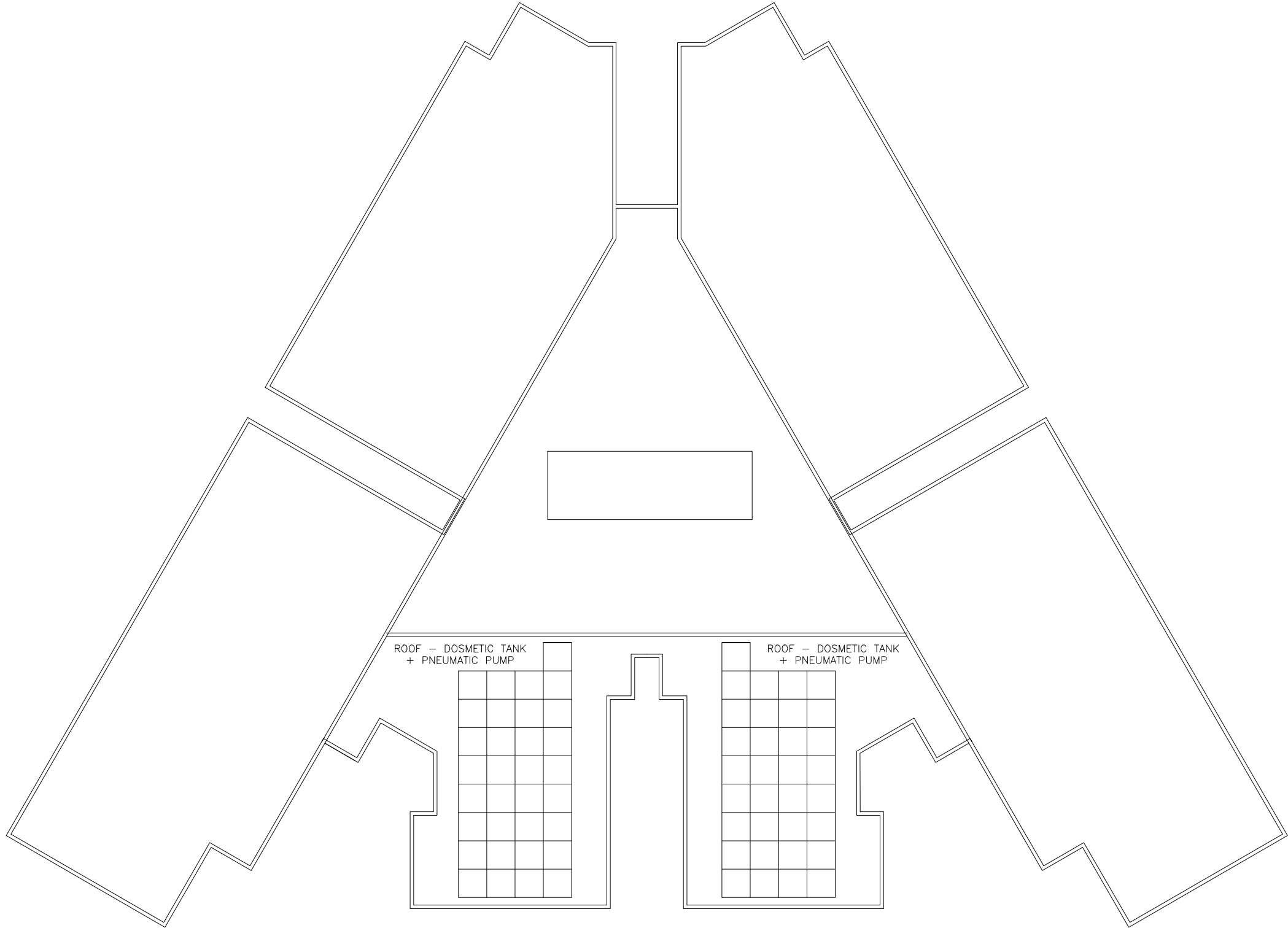
SERVICE APARTMENT _ROOF PLAN scale 1: 200
