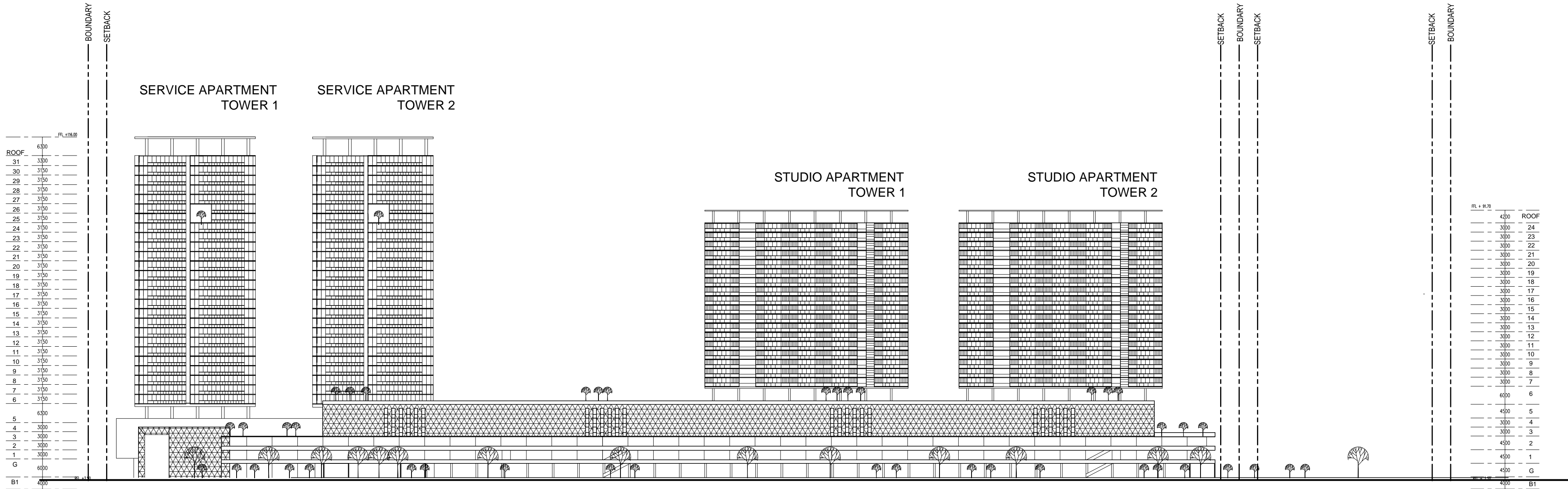
ELEVATION 02 scale 1:1000
