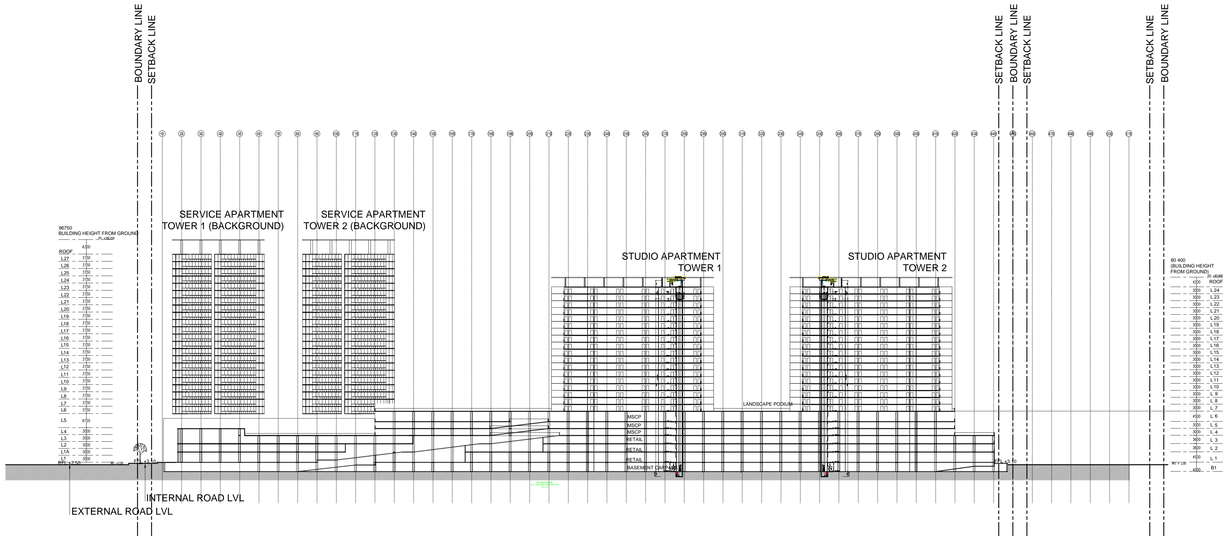
SECTION B-B' scale 1:1000
