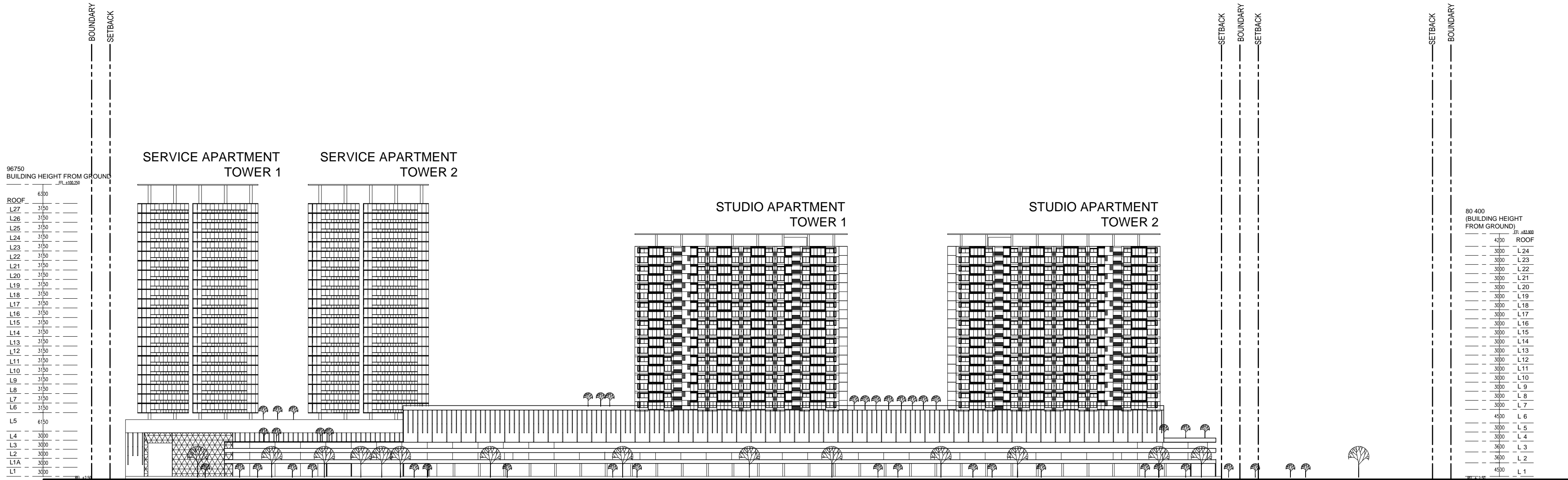
ELEVATION 02 scale 1:1000
