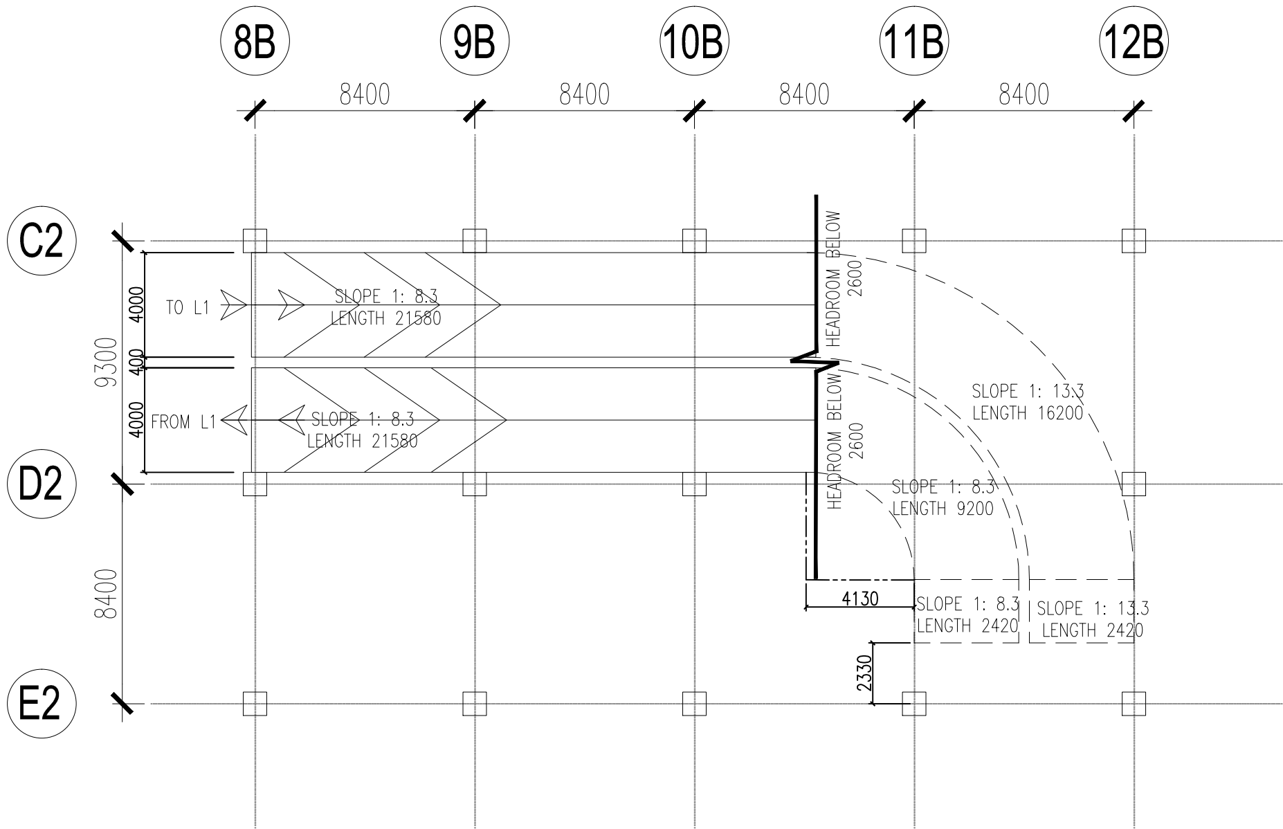
TYPE 1 (BASEMENT TO L1)
