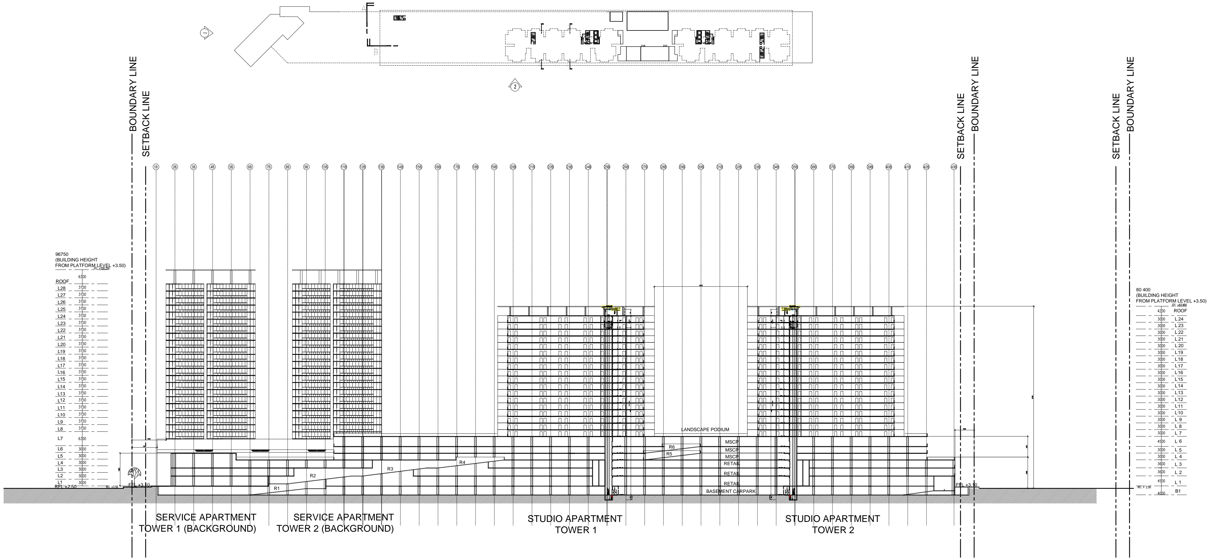
SECTION B-B'
