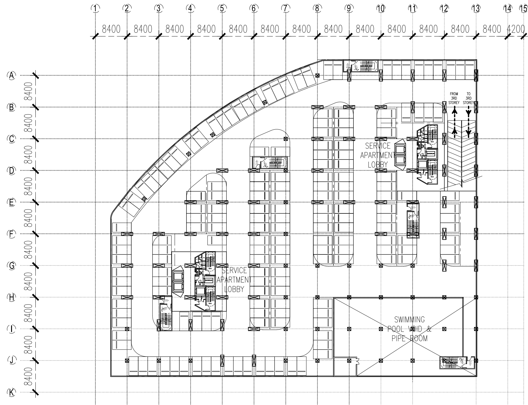
PLOT 01 - CAR PARK 4TH STOREY FLOOR PLAN
