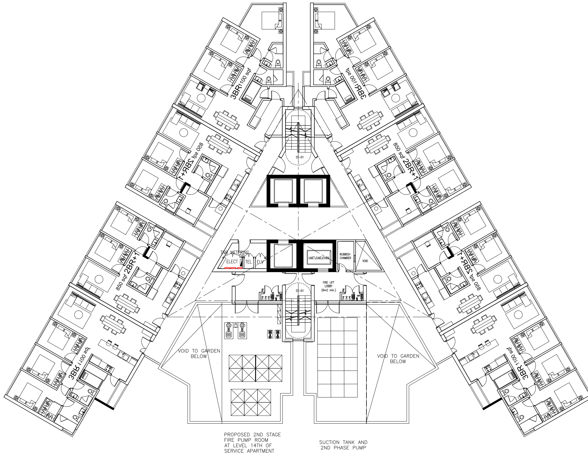
SERVICE APARTMENT_13TH FLOOR scale 1: 200
