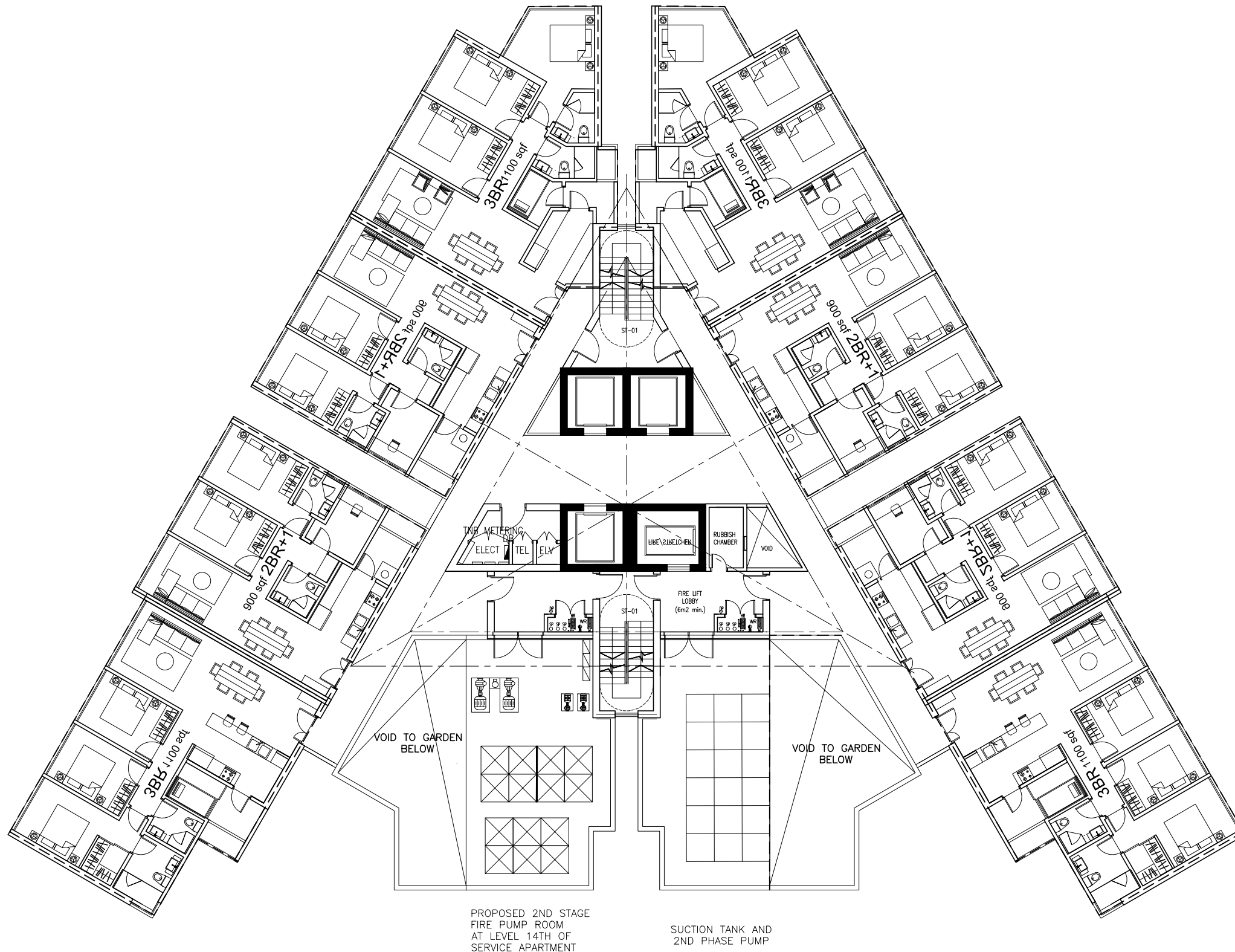
SERVICE APARTMENT_14TH FLOOR scale 1: 200
